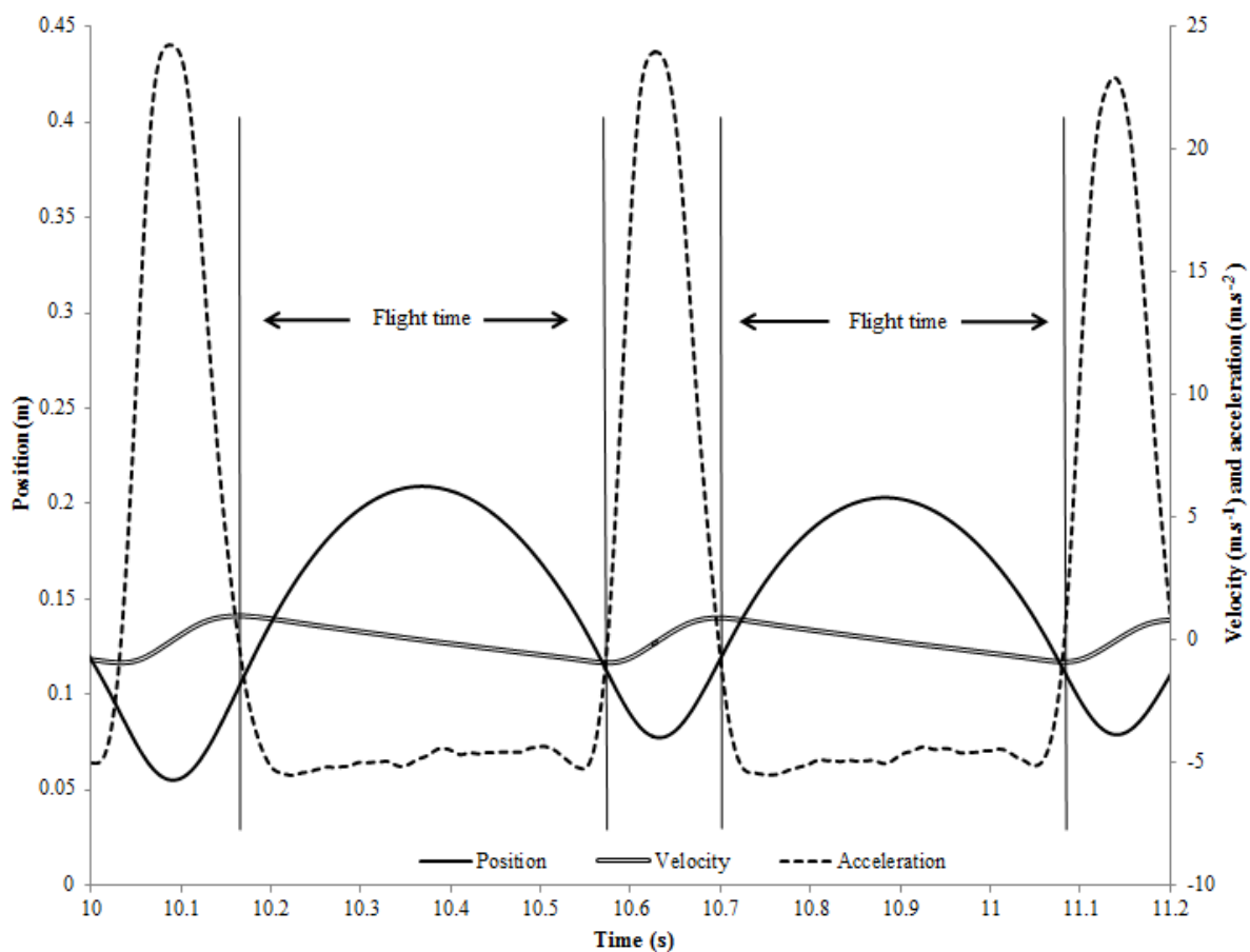
Figure 2. Calculation of CT and FT based on sledge marker kinematics. CT was defined as the time period when acceleration was greater than 0 m.s -2 , and FT as the time between consecutive CT (as shown).
