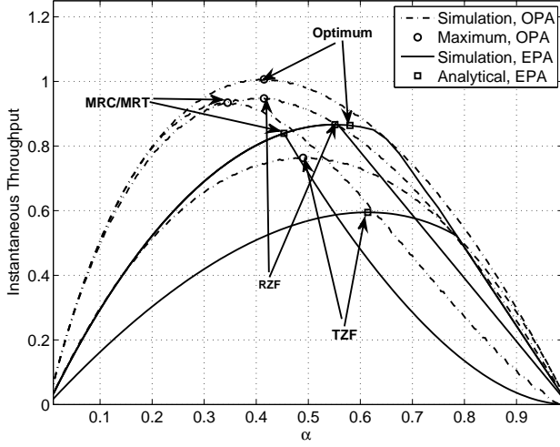
Fig. 2. Instantaneous throughput versus \alpha for proposed beamforming schemes ( M_T = M_R = 3 , P_S = 20 dBm, d_1 = 20 , d_2 = 10 and \tau = 3 ).
