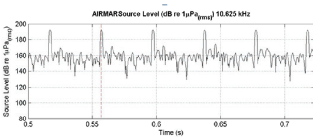
Figure 5: Effective RMS source level versus time at fundamental frequency. Duty cycle of around 3.5% during a burst sequence.
