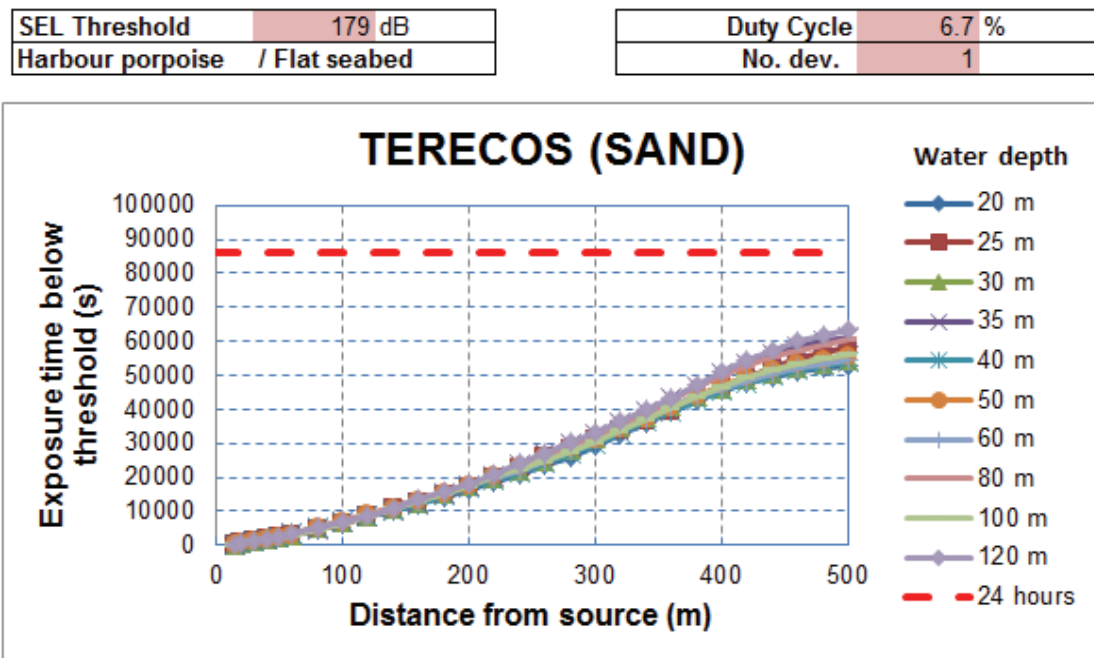
Figure 69b: Example output for time for exposure to reach the injury threshold of 179 dB re 1 \mu\text{Pa}^2\text{s} for a harbour porpoise for a single Terrecos system versus distance for multiple water depths.
