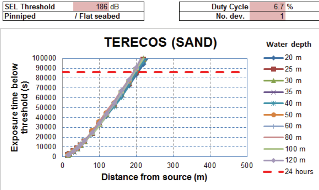
Figure 69a: Example output for time for exposure to reach the injury threshold of 186 dB re 1 \mu\text{Pa}^2\text{s} for a pinniped for a single Terrecos system versus distance for multiple water depths.
