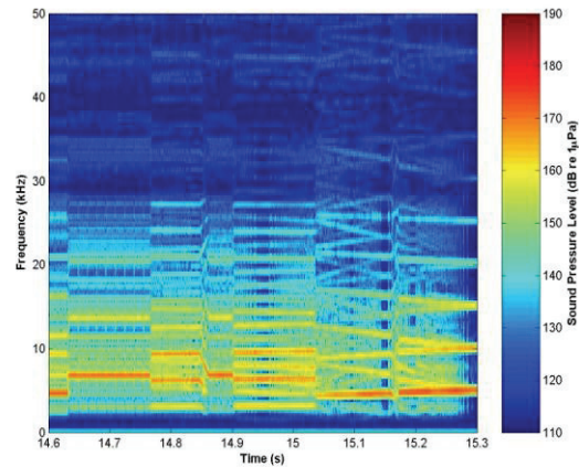
Figure 12: Terecos programme 2 spectrogram.
