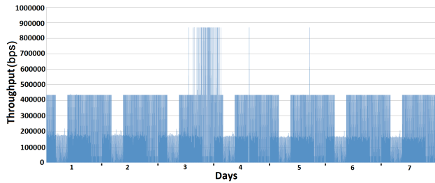
Figure 3. Throughput Measurements Over 7 Days - 168 Hours
