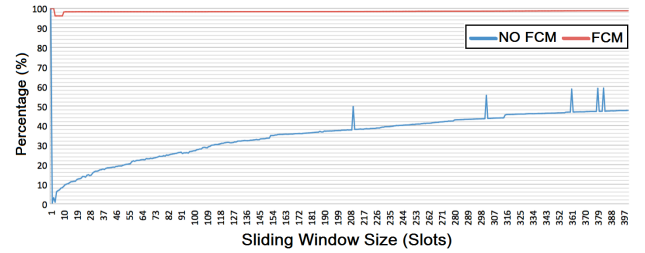
Figure 7. OSR Anomaly Detection Results
