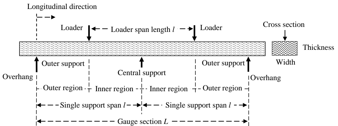
Figure 2: Loading and supporting of a composite beam in the DBS method
