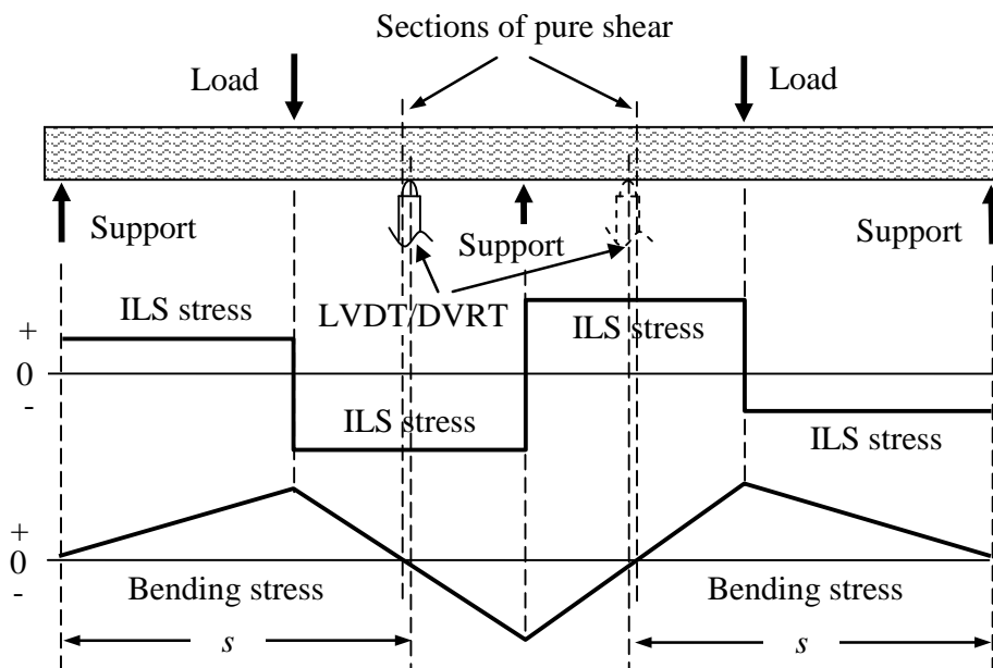
Figure 3: ILS and bending stress distributions in the DBS specimen
