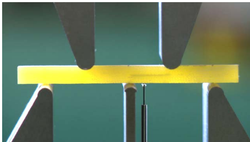
Figure 1: A test set-up of the DBS method
