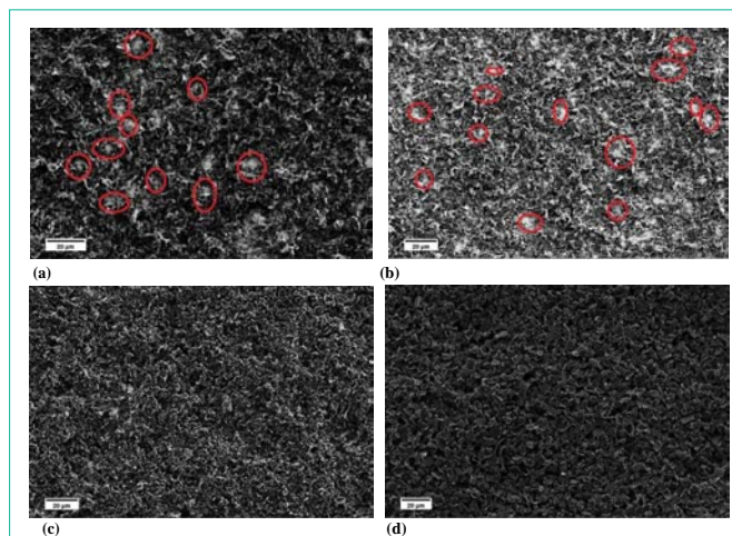
Figure 3: SEM images of the carbon based particles coated sample by EPD; (a) The PP10 coated sample with initial EDP conditions; (b) The PP10 coated sample with lower voltage; (c) The PP 10 coated sample with longer deposition time; (d) G coated sample with longer deposition time.
