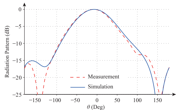
Fig. 6. Simulation and measured results for radiation pattern at 2.34 GHz, at \phi = 90^\circ cut plane.
