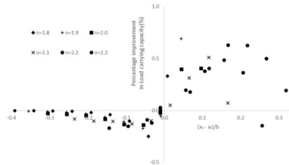
Figure 1: Percentage of improvement in load carrying capacity as a function of loci of recirculation boundary and texture positioning
