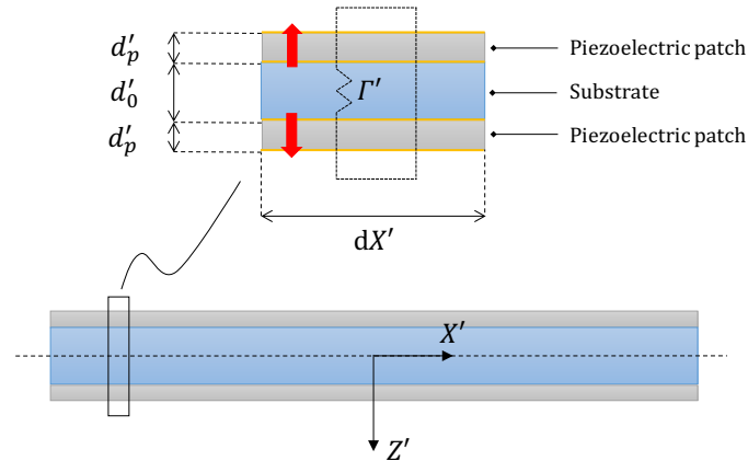
Figure 2. Geometry of the piezoelectric plate and detail of the bimorph configuration for an element of length dX' \ll L' , corresponding to the length of a piezoelectric patch. The bold vertical arrows indicate the poling direction of the piezoelectric layers (from negative to positive pole). Electrodes of negligible thickness cover both faces of each piezoelectric patch. Each pair of piezoelectric patches are shunted with an external resistance 1/\Gamma' , thus powering a resistive circuit.
