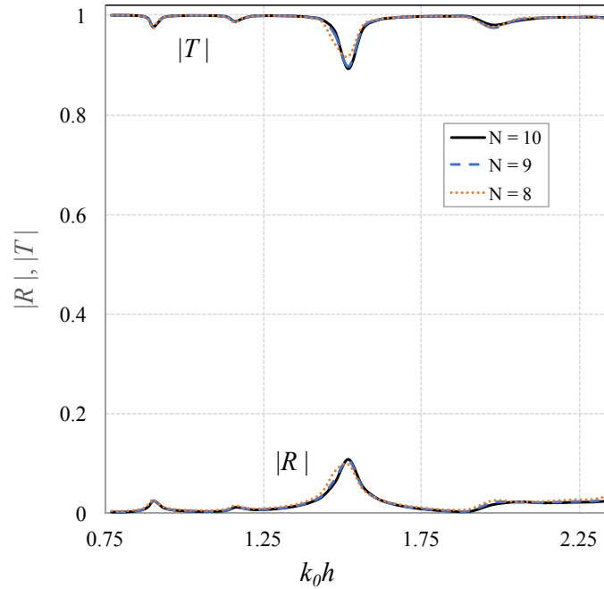
Figure 8. Behaviour of the transmission (upper line) and reflection (lower line) coefficients with respect to the non-dimensional parameter k_0 h , for three different values of N . The maximum combined error for N = 9 is O(10^{-3}) .
