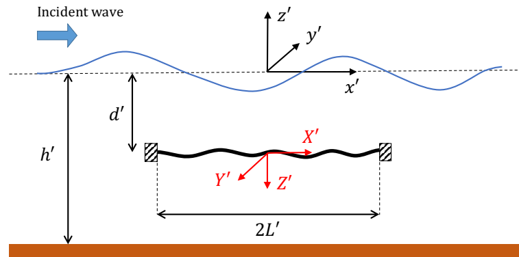
Figure 1. Geometry of the system in physical variables. The local reference system on the plate is (X', Y', Z') and the global coordinate system is (x', y', z') . The plate is long 2L' and is clamped at both ends at a depth d' in an ocean of constant depth h' .
