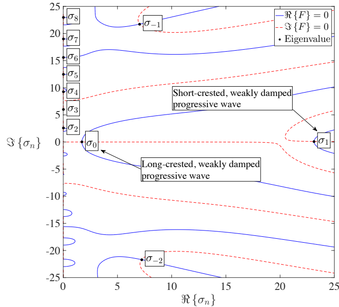
Figure 4. Location of the first 11 eigenvalues of the hydro-electromechanical dispersion relation F(\sigma_n) = 0 in the complex \sigma_n plane, see (3.37). The solid blue lines identify the contours \Re\{F\} = 0 , while the dashed red lines correspond to the contours \Im\{F\} = 0 . The parameters are \alpha = 0.21 , \beta = 3.8 \times 10^{-4} and \xi = 1 .
