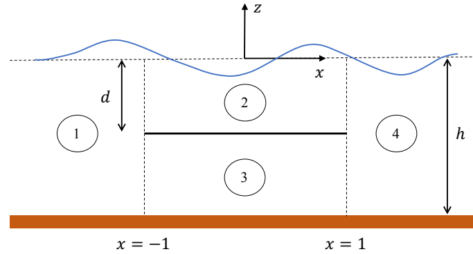
Figure 3. Domain decomposition used to solve the boundary-value problem (3.20)–(3.24).
