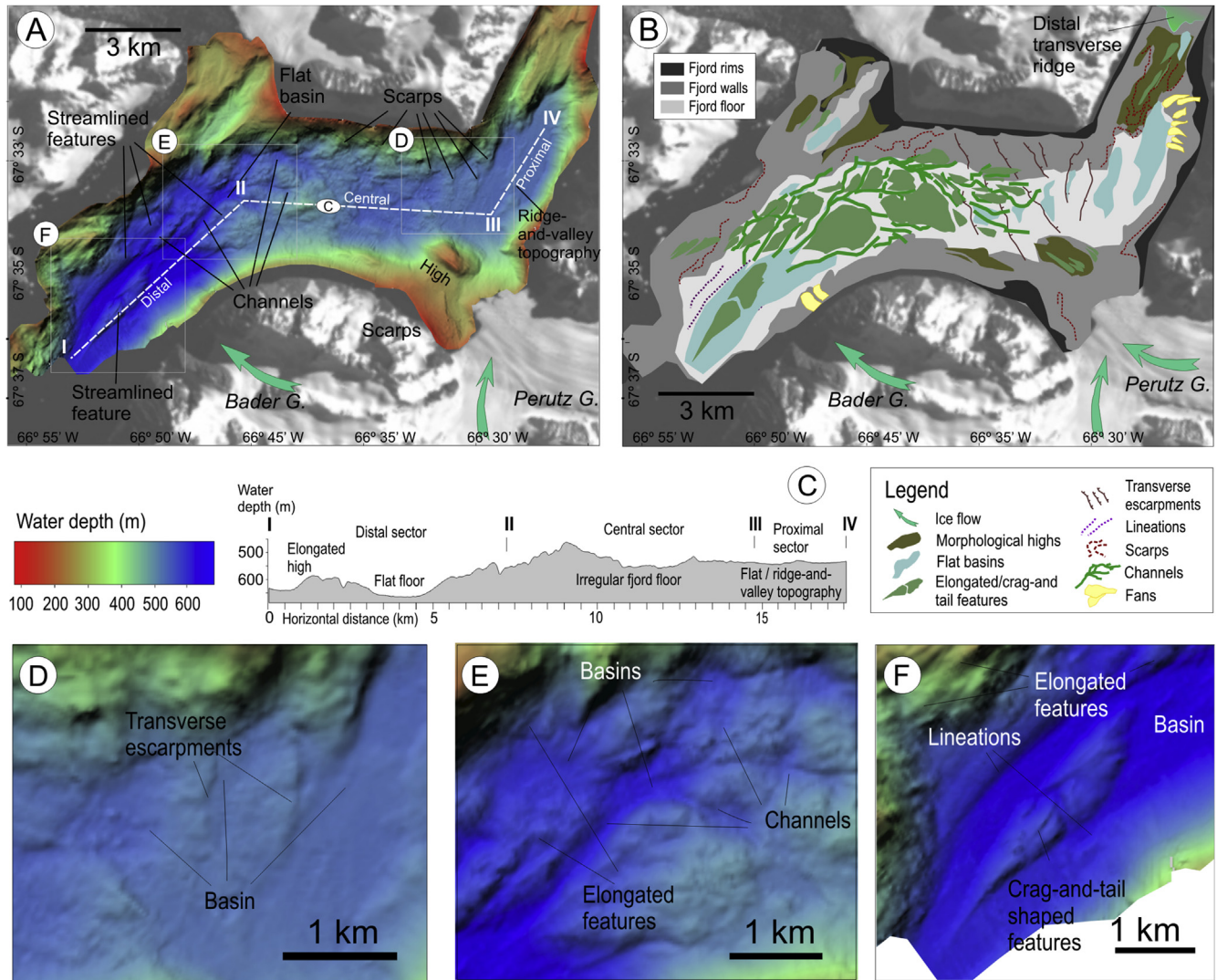
Fig. 3. Morphological characterization of the main Bourgeois Fjord and shallow areas off the tidewater glaciers draining into it. (A) Multibeam bathymetry. (B) Distribution of submarine landforms. (C) Bathymetric profile along the main fjord illustrating the seafloor relief along the proximal, central and distal sectors. (D) Transverse escarpments and basins. (E). Smooth sedimentary basins and bedrock channels. (F) Elongate features and streamlined lineations.
