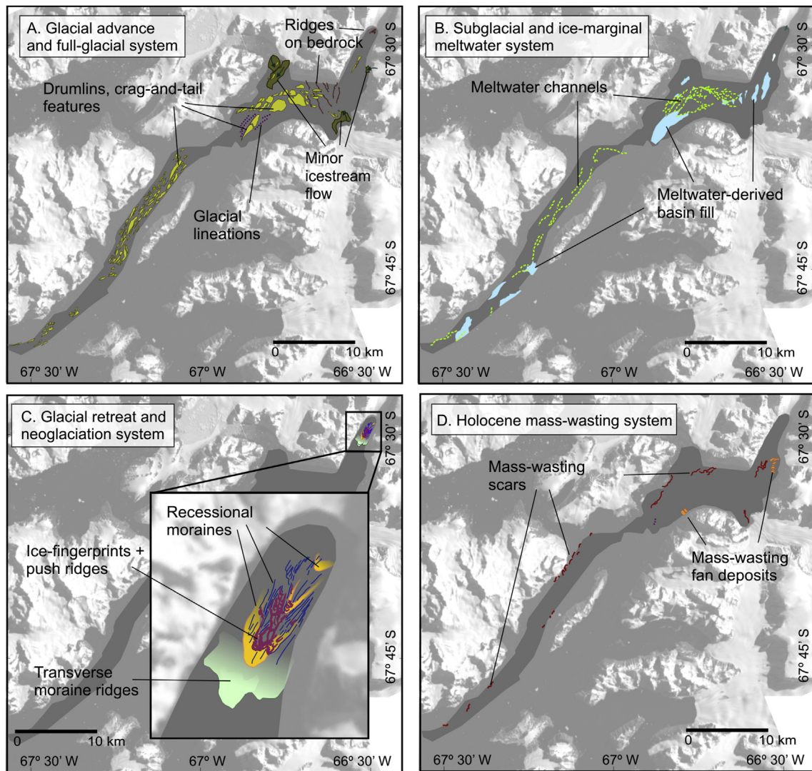
Fig. 9. Spatial distribution of the submarine landforms composing the four morpho-sedimentary systems in Bourgeois Fjord. (A) Glacial advance and full-glacial; (B) Subglacial and ice-marginal meltwater; (C) Glacial retreat and neoglaciation; and (D) Holocene mass-wasting.
