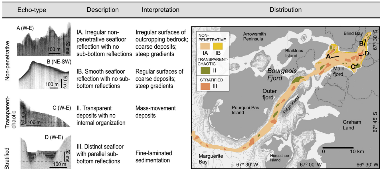
Fig. 2. Acoustic facies characterization, distribution and interpretation. Selected TOPAS profiles are shown to illustrate the acoustic character of each echo-type: non-penetrative, transparent-chaotic and stratified. Descriptions and interpretations are given, and follow the criteria first proposed by Damuth (1980) and further developed by Kuhn and Weber (1993) and Droz et al. (2001).
