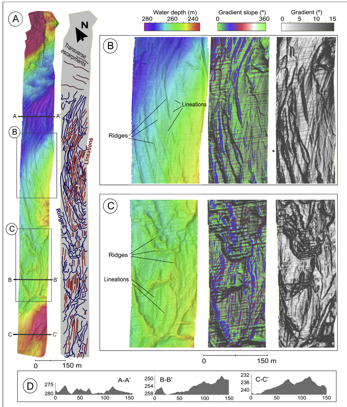
Fig. 6. Morphological characterization of the inner sector of Blind Bay, based on the Isis ROV high-resolution multibeam imagery. (A) Bathymetric mosaic and interpretation (located in Fig. 6A). (B) and (C) Detailed sections showing the bathymetry, gradient-slope direction and gradient of the area characterized by finger-like ridges and lineations. (D) Bathymetric profiles displaying the morphology of the ridges and lineations (axes in m).
