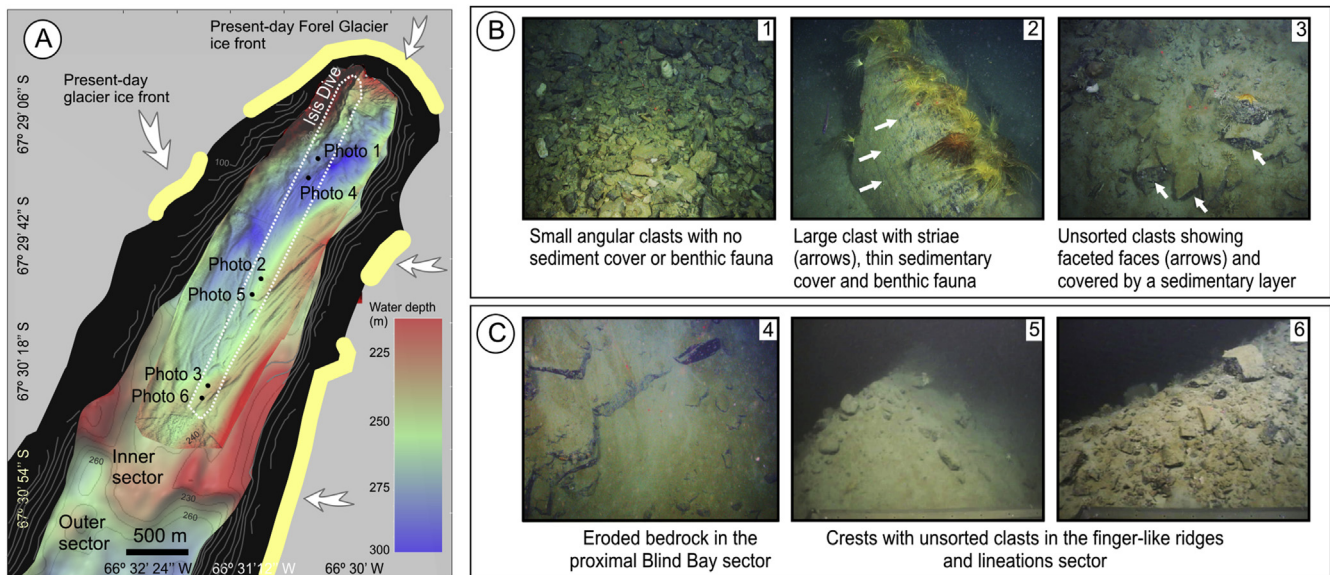
Fig. 7. ROV-acquired photographs of the seafloor along a transect in the inner sector of Blind Bay (locations of photographs shown in A). (B) Photographic transect from ice-proximal (Photo 1) to distal positions (Photo 3) along the inner part of Blind Bay. (C) Photographs illustrating the erosional character of the proximal area (Photo 4) and the morphological crests in the distal area representing finger-like ridges and lineations (Photos 5 and 6).
