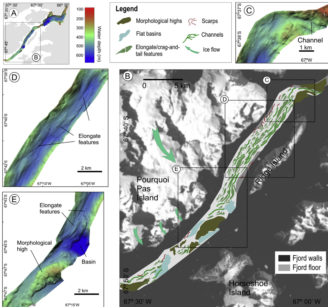
Fig. 4. Morphological characterization of outer Bourgeois Fjord. (A) Location map. (B) Distribution of submarine landforms inferred from multibeam bathymetry data. (C) to (E) Detailed bathymetric mosaics illustrating the morphological characteristics of channels, streamlined features and smooth basins identified in the outer fjord (located in B).
