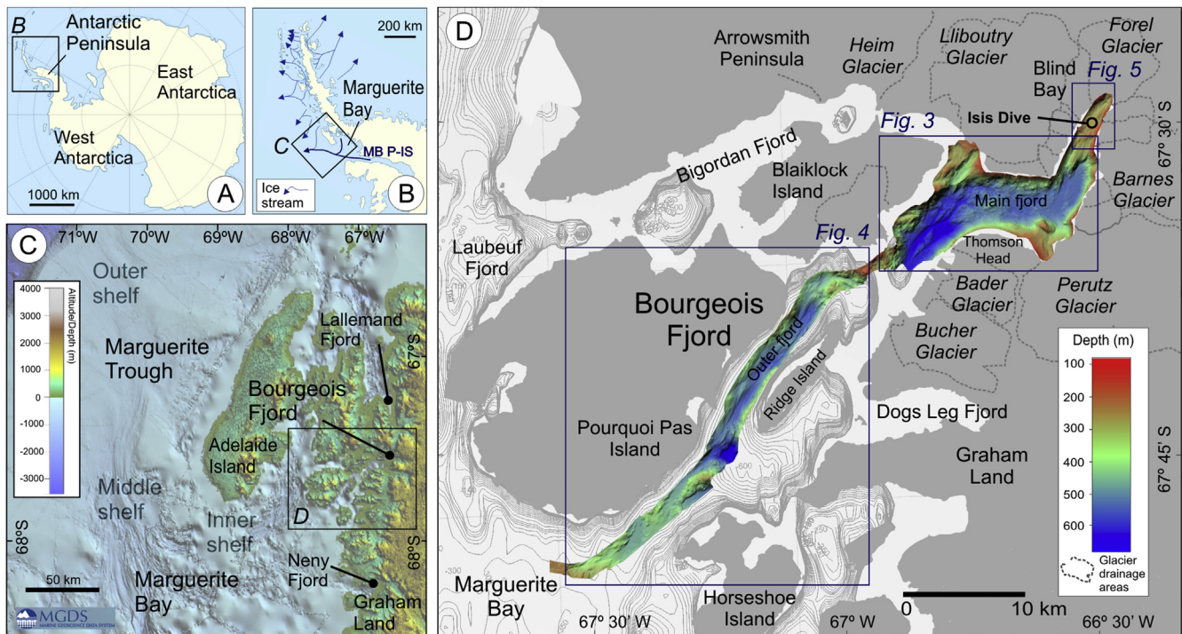
Fig. 1. Study area, in Marguerite Bay, Antarctic Peninsula (A). (B) Palaeo-ice streams of the Antarctic Ice Sheet during the last glacial period around the Antarctic Peninsula, from Livingstone et al. (2012). MB P-IS: Marguerite Bay palaeo-ice stream; (C) Regional topographic map of Marguerite Bay (data from the Marine Geoscience Data System; http://www.marine-geo.org ). Neny and Lallemand Fjords, located in neighbouring areas of the Antarctic Peninsula are shown. (D) Bathymetry of Bourgeois Fjord on the Pacific side of the Antarctic Peninsula. The limits of glaciers on Graham Land and the islands have been mapped from the LIMA satellite-image mosaic provided by the USGS EROS Center. The map shows the location of the Isis ROV dive in Blind Bay, off Forel Glacier and the bathymetry of the main and outer Bourgeois Fjord from our multibeam data.
