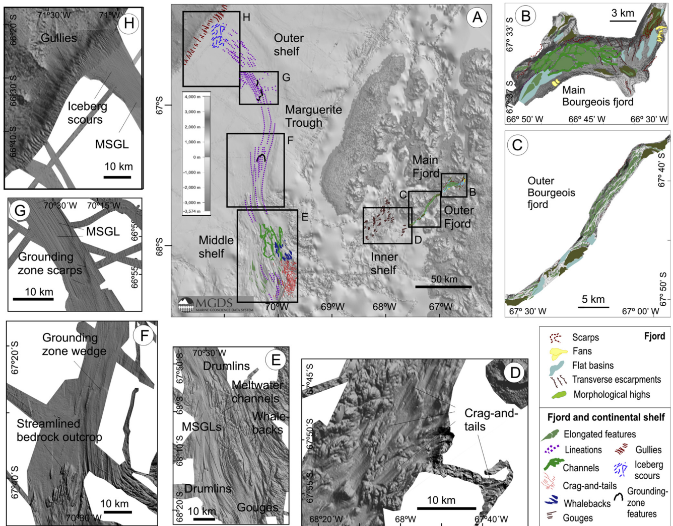
Fig. 8. (A) Regional map of Marguerite Bay showing the landforms assemblage as discussed in this work, integrated with the results from Dowdeswell et al. (2004a,b), Ó Cofaigh et al. (2005) and Livingstone et al. (2013). (B) to (H) Greyscale seafloor bathymetric models (see location in (A)) showing the detailed characteristics and distribution of the landforms. Regional bathymetric data have been obtained from the Marine Geoscience Data System ( http://www.marine-geo.org ).
