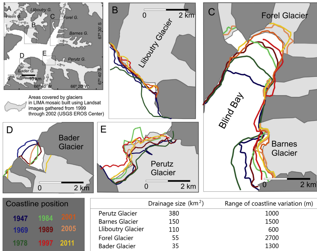
Fig. 10. Variations in the locations of tidewater-glacier margins between 1947 and 2011, inferred from maps, aerial photographs and satellite images. The figure illustrates the different trends in terminus fluctuations different tidewater glaciers draining into Bourgeois Fjord.
