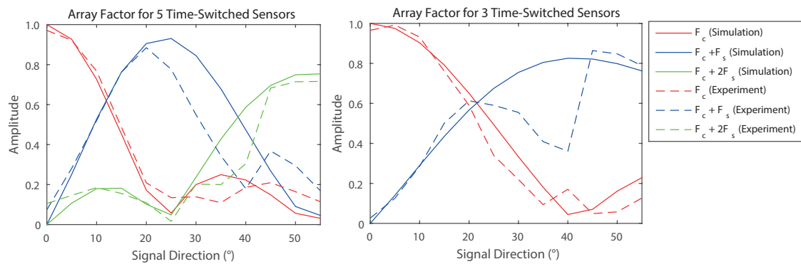
Figure 9. The received harmonic content of an experimental five-element linear microphone array compared to the expected numerical results.
