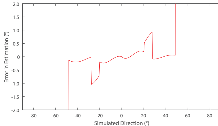
Figure 6. Simulated error in direction of arrival estimation when the best result is picked from a linear array using five or three of its elements.
