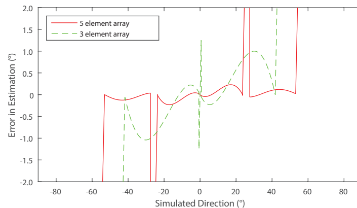
Figure 5. Simulated error in direction of arrival estimation of a linear array using five (solid) or three microphones (dashed).
