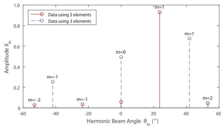
Figure 4. Power spectrum produced by a five-element array receiving a signal from a source at an angle of 25^\circ . When the samples from the outer elements are removed, then the array produces a new spectrum with different characteristics (shown as the dotted lines in the figure).
