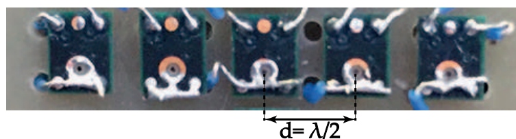
Figure 8. Setup of the experimental microphone array with an inter-element spacing ( d ) of approximately \lambda/2 where \lambda is the wavelength of a 40 kHz acoustic wave. Each microphone is a SPU0410LR5H-QB [18] Micro-Electromechanical Systems (MEMS) omnidirectional microphone.
