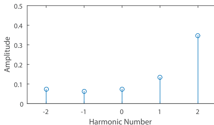
Figure 3. Power spectrum produced by a single sinusoidal source when sampled by a uniformly switched five-element time modulated linear array. The signal is impinging on the array at an angle of 45^\circ .
