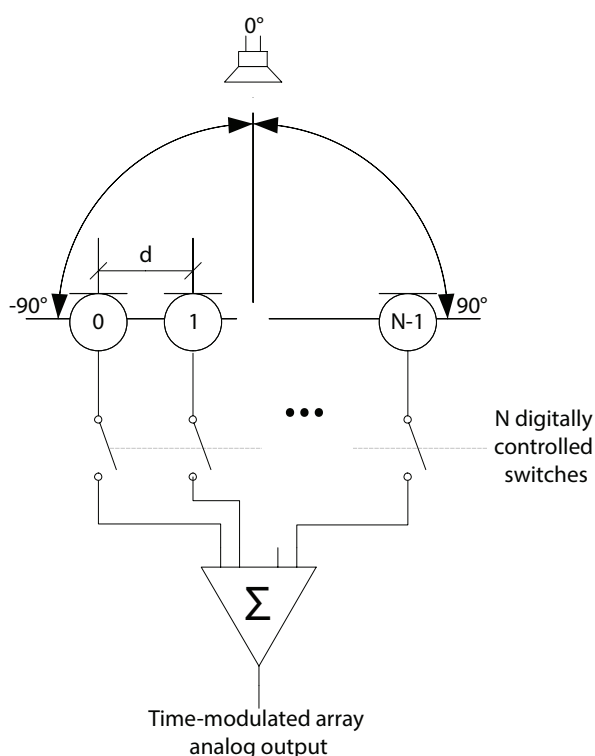
Figure 1. Typical schematic of an N element time-modulated array with d spacing.
