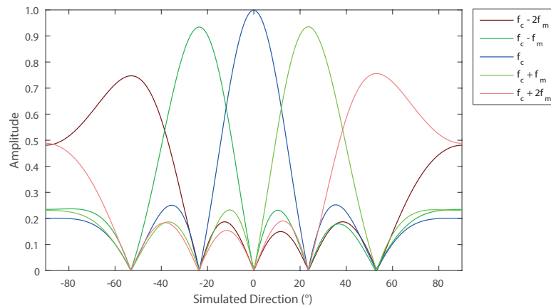
Figure 2. Simulated Array Factor of a five-element array, for five different harmonics when each element is switched on and off uniformly in sequence.
