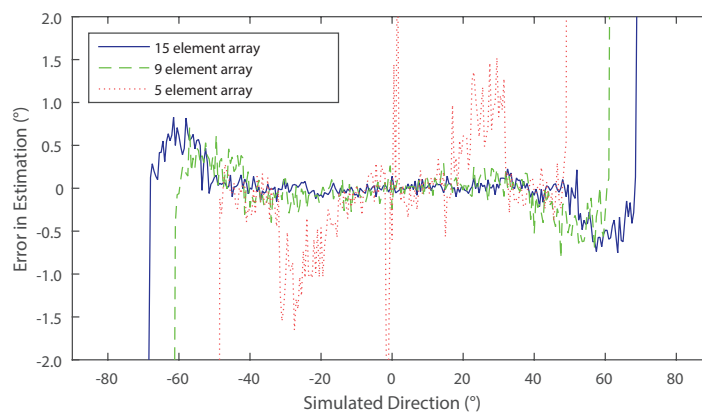
Figure 7. Simulated error in direction of arrival estimation with three different numbers of elements in the presence of noise. Each test had 1350 samples taken from an array with five (dotted), nine (dashed) or fifteen (solid) elements, where the source signal to noise ratio was 10 dB.
