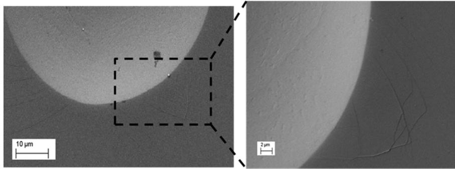
Figure 3: SEM images of micro-indentation in Zr_{48}Cu_{36}Al_8Ag_8 .
