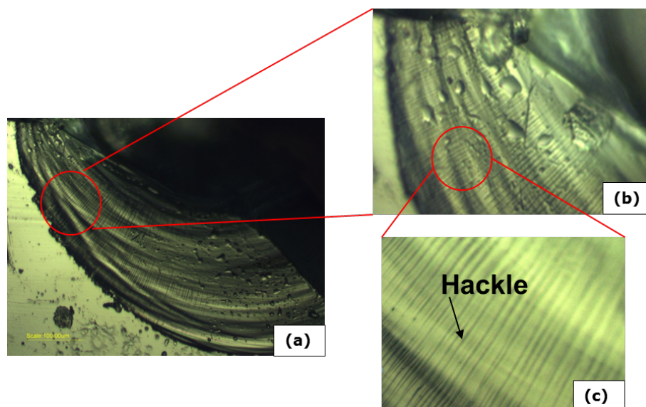
Figure 5: Optical micrographs of indented soda-lime-silica glass after applying 1.3 kN showing cone fracture form (a) and hackle fracture (b and c).
