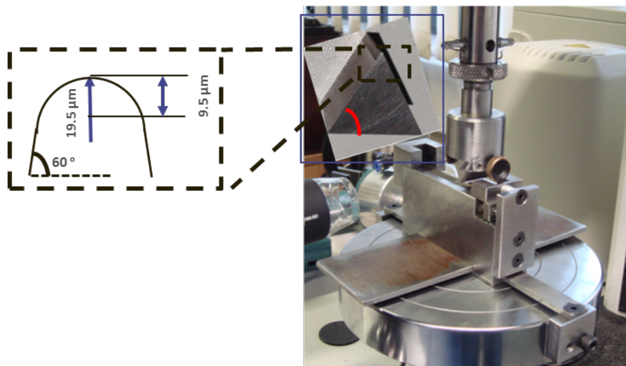
Figure 1: Experimental set-up for wedge indentation and its dimension
