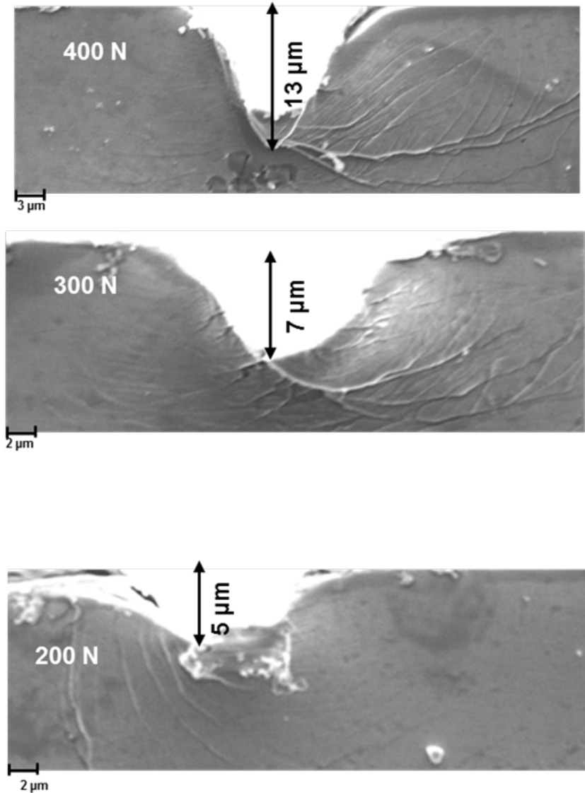
Figure 4: Evolution of shear bands pattern with load under wedge indentation: (a) 400 N, (b) 300 N, (c) 200 N.
