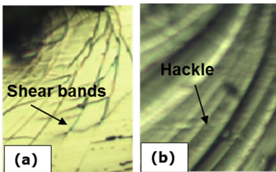
Figure 6: Optical micrograph of 1 kN wedge indentation on as-cast Zr_{48}Cu_{36}Al_8Ag_8 metallic glass (a) and soda-lime-silica glass (b).
