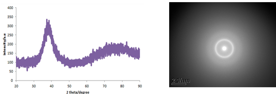
Figure 2: (a) XRD pattern of as cast Zr_{48}Cu_{36}Al_8Ag_8 , (b) corresponding SAED patterns.
