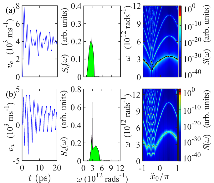
FIG. 6: (color online). A typical time-realization of v_a(t) (left panel), its Fourier spectrum S_a(\omega) (middle panel) and the dependence of the spectrum S(\omega) on the initial position of the particle x_0 (right panel) calculated for (a) U = 1.5 meV < U_{cr1} and (b) U = 3.45 meV > U_{cr1} . Dot-dashed lines mark the dependence \omega_1(x_0) calculated analytically (see the text for details). The spectra in the right panels are given in log-scale in order to make the spectral peaks more noticeable.
