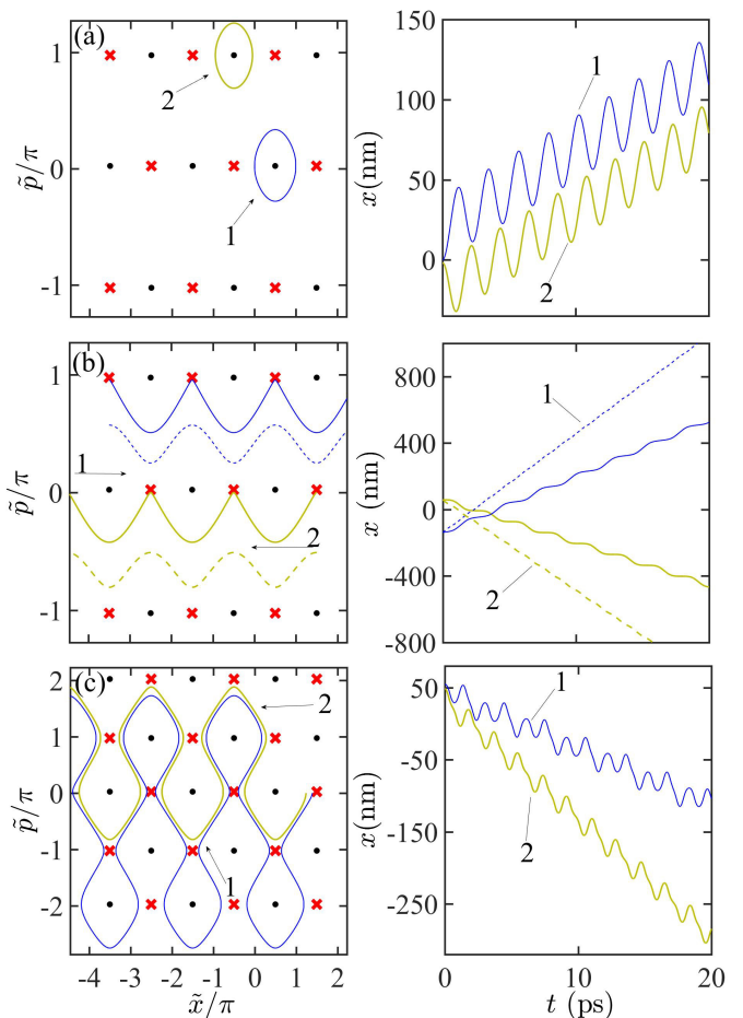
FIG. 5: (color online). Three distinct types of the phase trajectories (left panels) and the corresponding electron trajectories in the real space (right panels) for (a) U = 1.5 meV; (b) U = 2.5 meV; (c) U = 4.2 meV.
