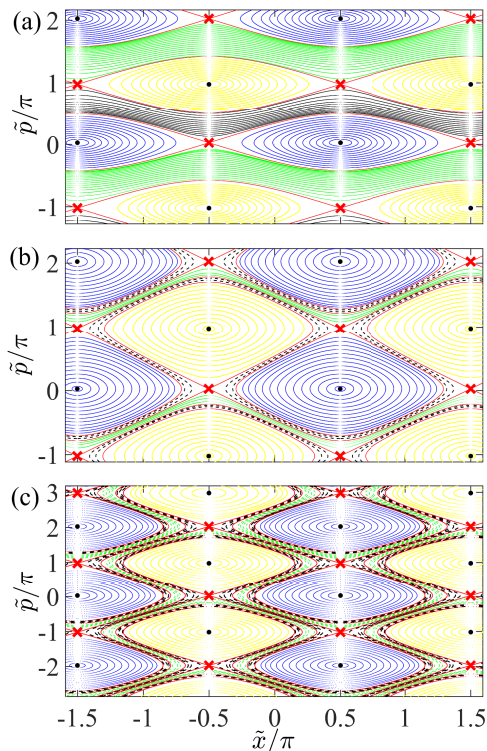
FIG. 2: (color online). Phase portraits of the dynamical system (8) for (a) U = 1.5 meV ( U < U_{cr1} ); (b) U = 3.45 meV ( U > U_{cr1} ) and (c) U = 4.25 meV ( U > U_{cr2} ). The positions of equilibrium points are indicated by black solid circles (centres) and red crosses (saddles). The localized orbits are represented by blue and yellow dots. Smooth solid curves correspond to the unbounded trajectories, dashed curves mark the meandering trajectories, and red curves denote the separatrices.
