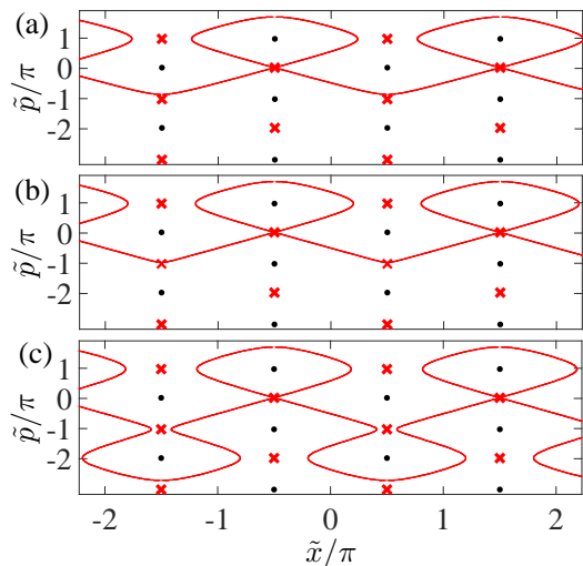
FIG. 4: (color online). Evolution of the separatrix structure with a variation of U in the vicinity of the second bifurcation ( U_{cr2} = 3.92 meV): (a) U = 3.7 meV; (b) U = 3.9 meV; (c) U = 4 meV. Other notations are the same as in Fig. 3.
