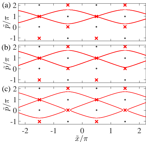
FIG. 3: (color online). Evolution of the separatrix structure with a variation of U around the first bifurcation point ( U_{cr1} = 3.1 meV): (a) U = 2.5 meV; (b) U = 3 meV; (c) U = 3.15 meV. The positions of the centres are indicated by black solid circles and the saddles – by red crosses.
