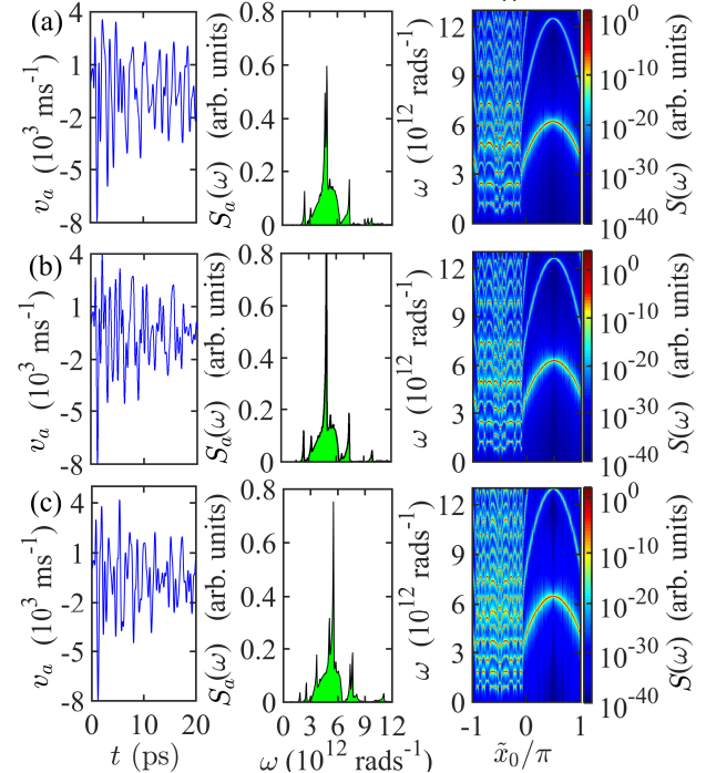
FIG. 7: (color online). A typical time-realization of v_a(t) (left panel), its Fourier spectrum S_a(\omega) (middle panel) and the dependence of the spectrum S(\omega) on the initial position of the particle x_0 (right panel) calculated for (a) U = 4.85 meV, (b) U = 4.932 meV, and (c) U = 5.2 meV. The spectra in the right panels are given in log-scale in order to make the spectral peaks more noticeable.
