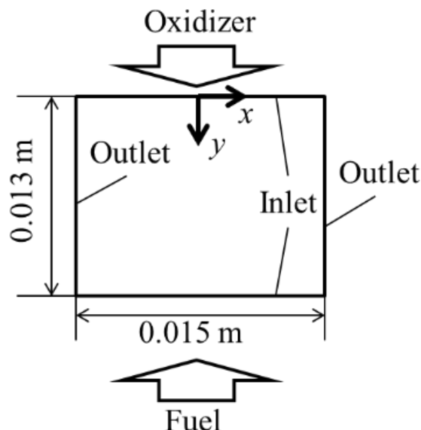
Figure 2. Analytical object for the simulation.
