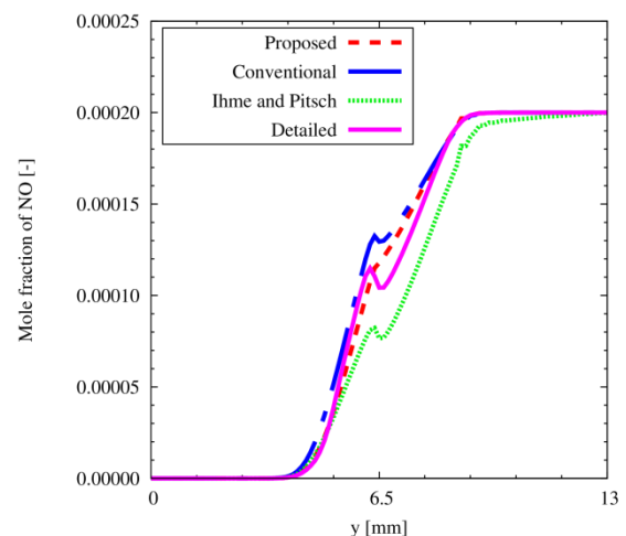
Figure 5. NO mole fraction distribution calculated with the proposed, conventional, Ihme and Pitsch's method, and the detailed chemistry model on y axis in the case 2.
