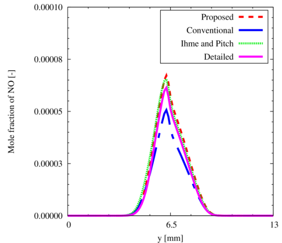
Figure 4. NO mole fraction distribution calculated with the proposed, conventional, Ihme and Pitsch's method, and the detailed chemistry model on y axis in the case 1.
