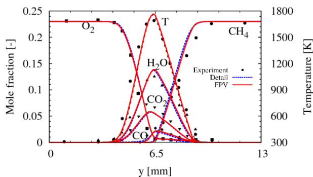
Figure 3. Temperature and major species profiles computed with the FPV or detailed chemistry model and the results of compared with the experimental data [10]
