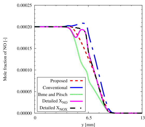
Figure 6. Comparison between the computed profiles of \text{NO} mole fraction distribution with the proposed, conventional, and Ihme and Pitsch's method, and mole fraction distribution of \text{NO} and \text{NO}_x calculated with the detailed chemistry model in the case 3.
