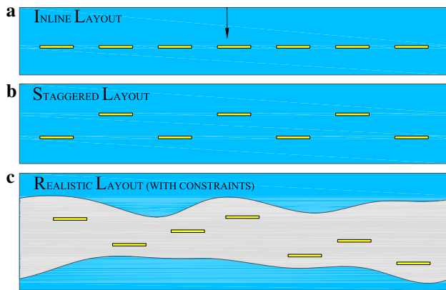
Fig. 11 Finite array of OWSCs. a Inline layout (2-D symmetry and uniform spacing); b staggered layout (1-D symmetry and uniform spacing); c a realistic wave energy farm layout
