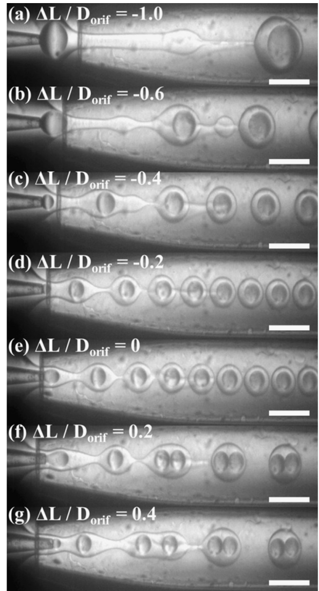
Fig. 7. The effect of distance between the two inner capillaries, \Delta L , on the generation of double emulsion drops. Q_1 = 2 mL/h, Q_2 = 7 mL/h, Q_3 = 35 mL/h, \rho_1 = 1012 kg/m 3 , \rho_2 = 940 kg/m 3 , \rho_3 = 1107 kg/m 3 , \mu_1 = 1.2 mPa s, \mu_2 = 10.4 mPa s, \mu_3 = 7.9 mPa s, \sigma_{12} = 29.9 mN/m, \sigma_{23} = 31.8 mN/m, D_{\text{orif}} = 376 \mu\text{m} , and D_N = 50 \mu\text{m} . All the scale bars are 400 \mu\text{m} .
