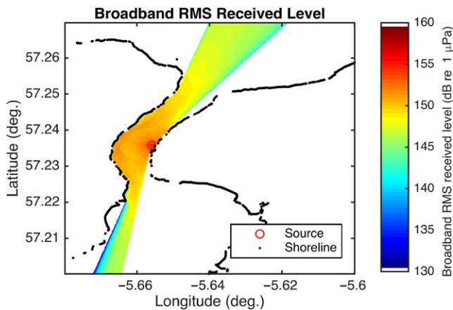
FIGURE 3 An example of the spatial variation in the modelled broadband received levels (dB re 1 \mu\text{Pa}_{(\text{RMS})} ) across the study area during periods with wind speeds of 0 m/s and a tidal height of 0 m above chart datum
