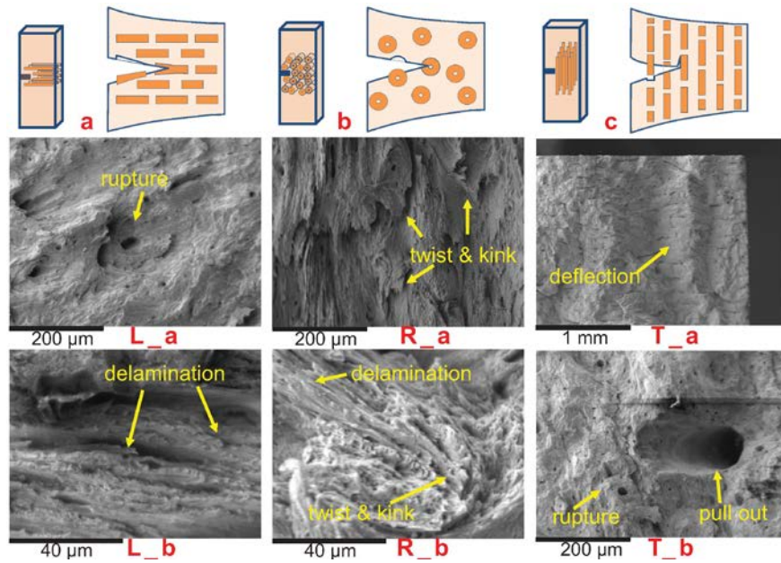
Fig. 5 Schematic illustrations and SEM images of various toughening mechanisms for longitudinal (a), radial (b) and transverse (c) cracks-growth directions, Labels at the bottom of each image indicate the corresponding magnified areas in Fig. 4
