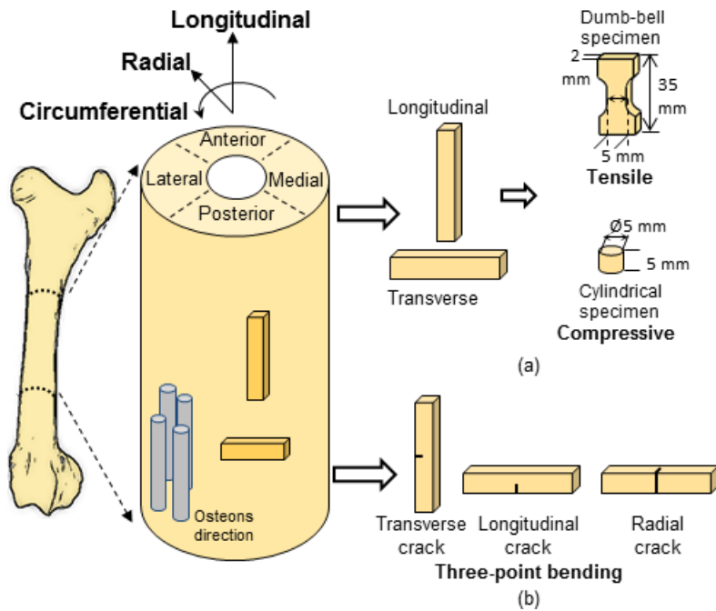
Fig. 1 Schematic illustration of specimen-preparation process for: (a) uniaxial tension and compression tests; (b) three-point bending tests
