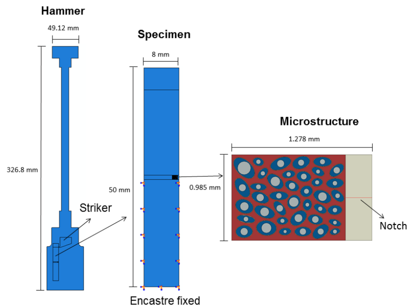
Fig. 6 Schematic illustrations of model configurations for Izod impact testing using microstructured bone model
