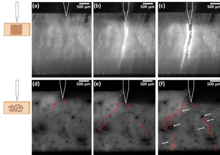
Fig. 10 High-speed-camera images of distinct damage processes in cutting parallel to osteons' direction,,: (a-c) C-L direction; (d-f) C-R direction; white lines designate profile of razor blade, red dotted lines indicate crack path and white arrows point at positions of osteons
