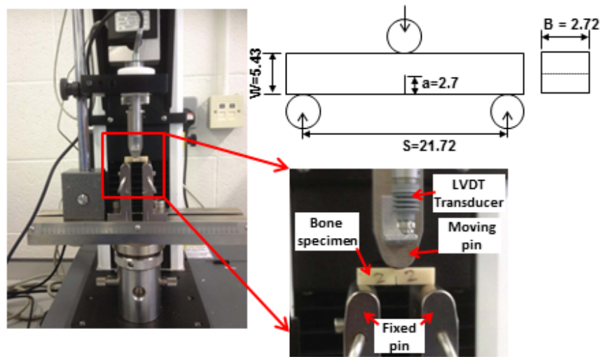
Fig. 3 Three-point bending test with single-edge-notch cortical-bone specimen and LVDT mounted on Instron 3345
