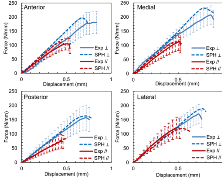
Fig. 11 Force (per unit width) – displacement diagrams for cutting of cortical bone in different orientations across four cortices; \perp and \parallel denote penetration perpendicular and parallel to osteons' direction, respectively
