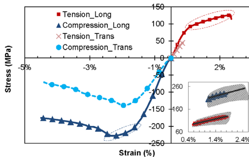
Fig. 2 Typical stress-strain curves for longitudinal and transverse specimens in tension and compression (anterior quadrant); inserts show strengthening portions for longitudinal specimens
