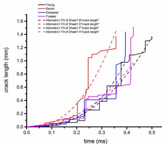
Fig. 8 Typical crack evolution curves for different micromorphologies
