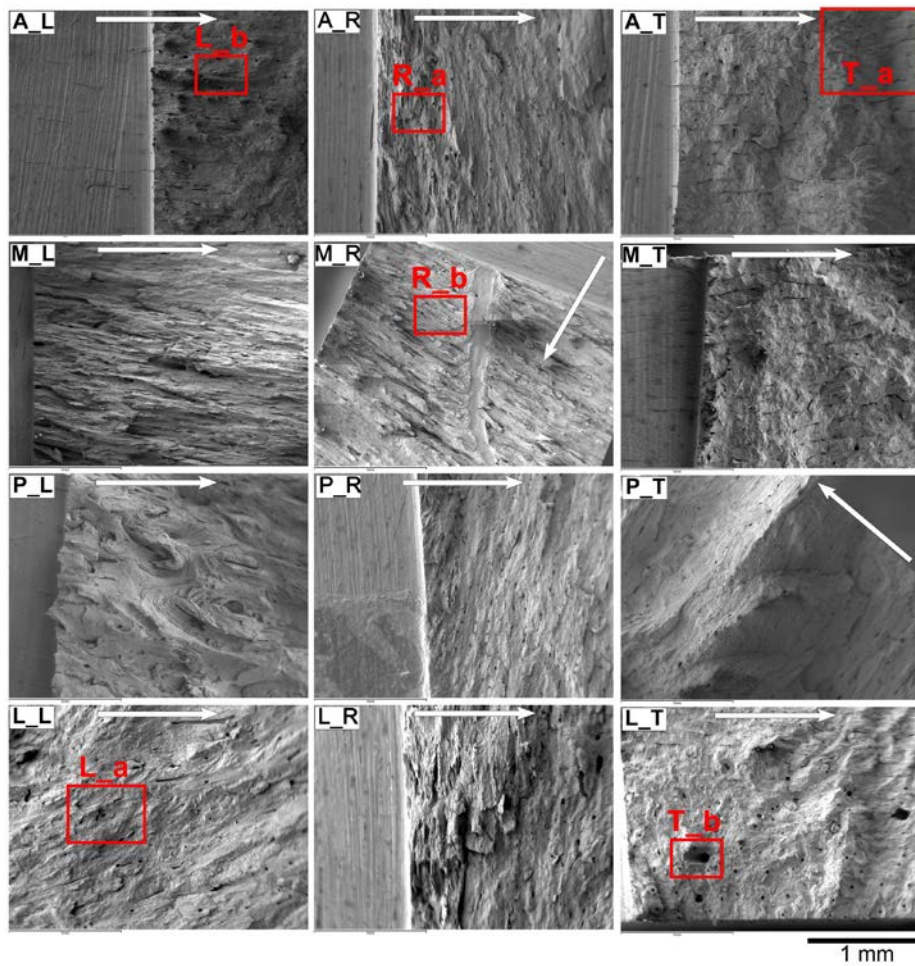
Fig. 4 SEM images of fracture surfaces for various cortex positions and crack propagation directions: A, M, P, L denote anterior, medial, posterior and lateral; _L, _R, _T denote propagation directions for longitudinal, radial and transverse cracks, respectively; white arrows indicate crack-growth direction
