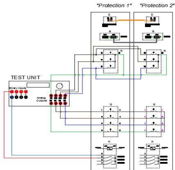
Fig. 1. Experimental test scheme.
