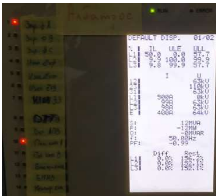
Fig. 4. Display of the IED.
