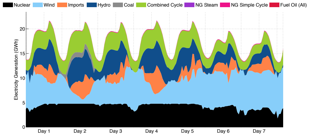
Figure 12: Modeled Electricity generation for a week in October by Generation Type
