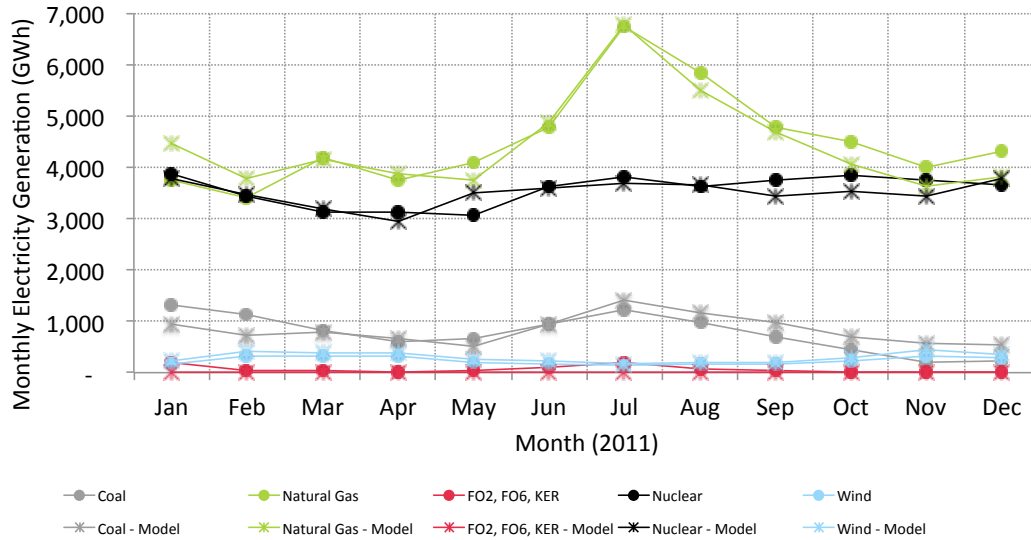
Figure 7: Comparison of monthly modeled electricity generation and reported electricity generation by fuel type
