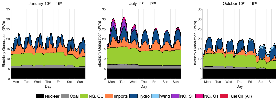
Figure 9: Hourly Modeled Generation by Generator and Fuel Type, 2011
