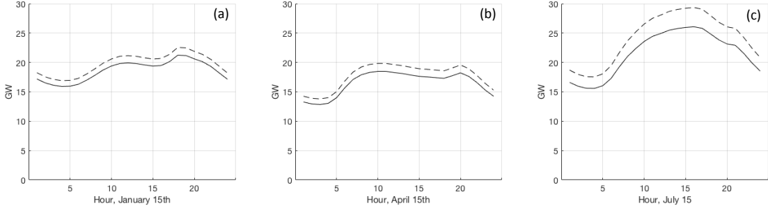
Figure 6: Hourly New York State Demand from 2011 (Solid) and projected for 2025 (Dotted). (a) January 15, Winter Period (b) April 15th, Swing Period (c) July 15th, Summer Period
