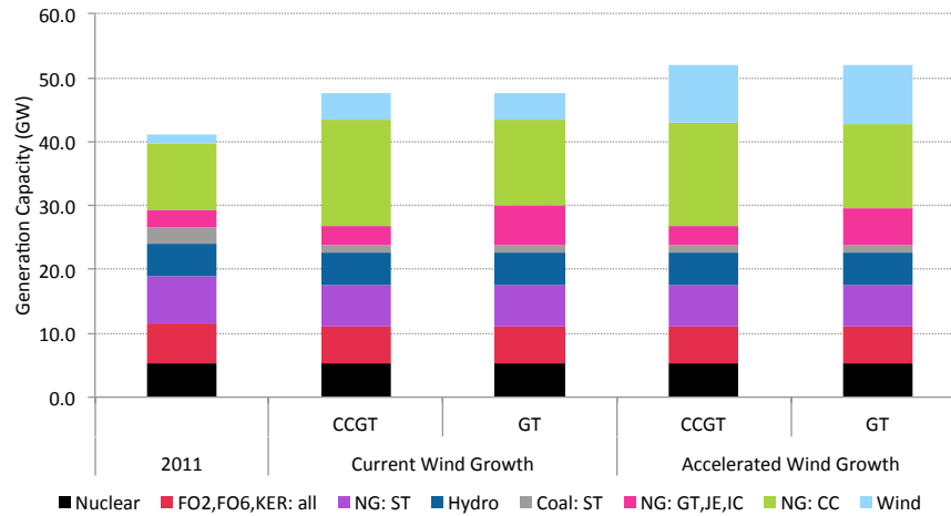
Figure 10: Total New York State Generation Capacity under all Generation Scenarios. Generation Capacity is indicated by fuel type and unit type
