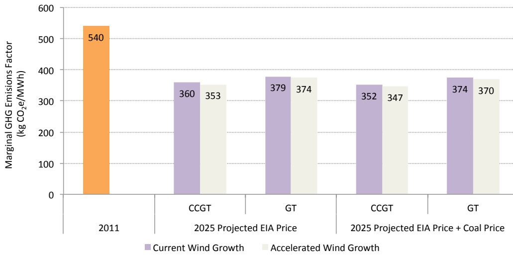
Figure 14: Marginal GHG Emissions Factors for New York City in 2025
