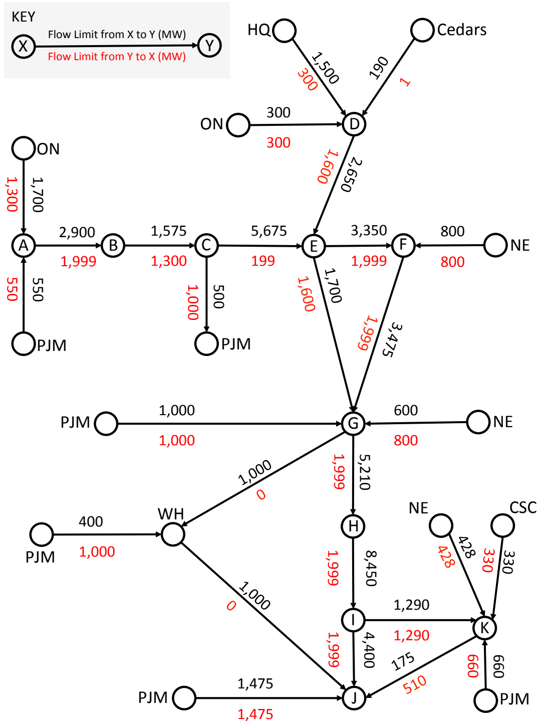
Figure 2: Transmission Network Topology with Maximum Flow Limits in (MW) between each zone and import region.
