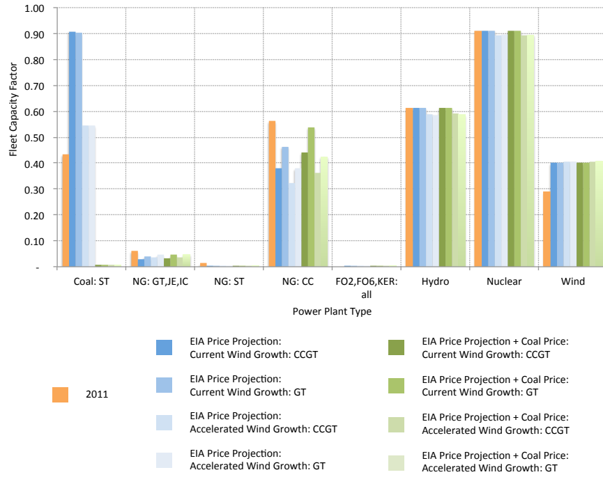
Figure 11: Annual Fleet Capacity Factors by Generation Type for Wind Growth, Makeup Generation, and Coal Price Scenarios
