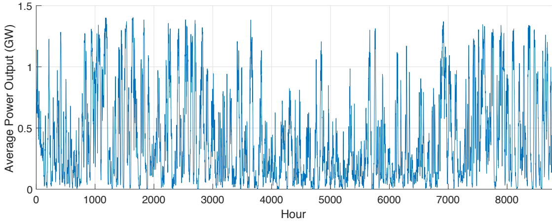
Figure 4: Aggregate Hourly Power Output of Wind Turbine Sites. Total Capacity: 1.4 GW
