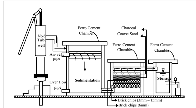
Figure 1. Flow Diagram of Community AIRP
