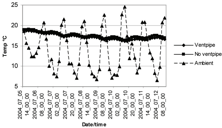
Figure 1. Vault A (with ventpipe) and vault B (no ventpipe): Heap temperatures 5 July - 12 July 2004
