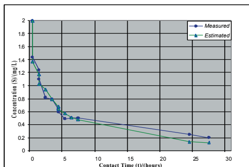
Figure 1. Measured and estimated concentration of fluoride
