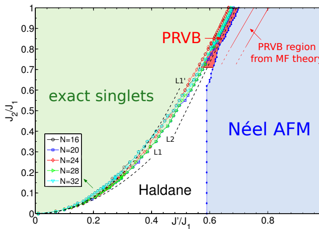
FIG. 2: (color online) The phase diagram of the present model obtained by exact diagonalizations (symbols with lines). The r lines enclose the stability region of the PRVB phase as obtained from the quadrumer boson operator method (see text). The dashed line L1 and L1' denote the boundary between the exact dimer and the Haldane phase as obtained from perturbation theory up to second and third orders, while the dashed line L2 is the line along which we examine the low-E spectrum shown in Fig. 5 below.
