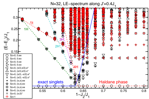
FIG. 4: (color online) Low-energy spectrum (measured from the GS) for the 32-site cluster along the line J'/J_1 = 0.4 in the S_z = 0 and 1 sectors. The blue solid line shows the energy of the exact singlet phase. The dashed lines highlight the n -Haldane chain singlets discussed in the text. The quantum numbers shown in the legends correspond to the allowed momenta of the 32-site cluster and the parities with respect to the two diagonal reflections \mathcal{R}_{1,2} .
