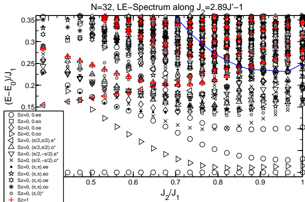
FIG. 5: (color online) Low-energy spectrum (measured from the GS) of the 32-site cluster along the line L_2 ( J_2 = 2.89J' - 1 ) of Fig. 2 in the S_z = 0 and 1 sectors. The solid (blue) line stands for the energy of the exact singlet phase.
