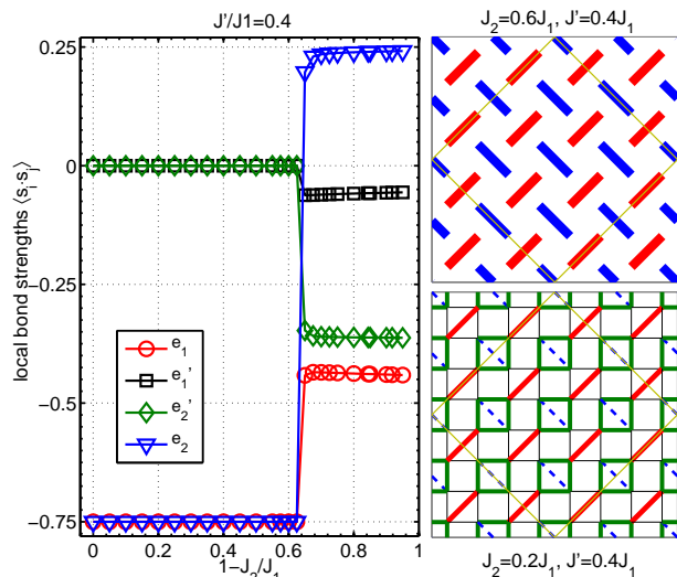
FIG. 3: (color online) Left panel: Ground state expectation values of the four different nearest-neighbor exchange energies \mathbf{S}_i \cdot \mathbf{S}_j for the 32-site cluster ( e_{1,2} for the J_{1,2} diagonal bonds, and e'_{1,2} for J' -bonds on plaquettes which contain J_{1,2} bonds). Right panels: The corresponding local energy profiles for representative cases inside the exact singlet state (above) and the Haldane state (below). Positive (negative) exchange values are shown by dashed (solid) lines, whose width is proportional to the magnitude of these values.
