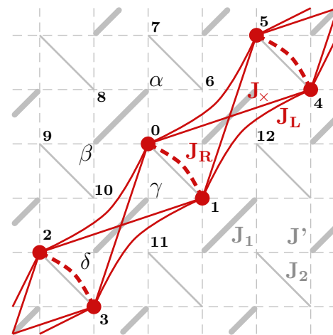
FIG. 1: (color online) The distorted SS model (thick and thin gray lines for J_1 , J_2 , and dashed for J' ) of this work, together with the effective quasi-1D model (red solid and dashed thick lines) emerging in the limit J_1 \gg J_2, J' which gives rise to the Haldane phase.
