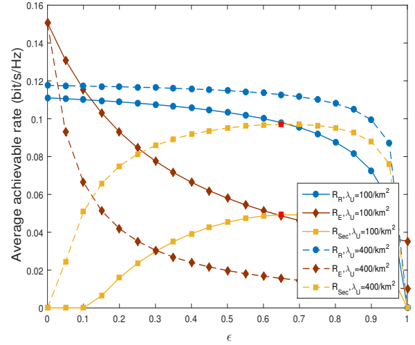
Fig. 9: The effects of the UAV jamming factor on the average rate, with P_U = 30 dBm, N_U = 4 , N_R = 16 , N_E = 4 and \lambda_E = 600/\text{km}^2 .
