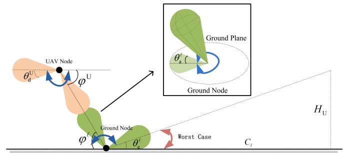
Fig. 2: Illustration of the antenna gain. As the figure shown, C_l is the maximum connection distance range for the ground node (eavesdropper shown), the black double sided arrow denoted the uniform range for depression angle \varphi^U and elevation angle \varphi^l range in [-\pi, 0] and [\frac{\theta_a^l}{2}, \pi - \frac{\theta_a^l}{2}] respectively. The sub figure shows the projection of 3D antenna beamforming, and the azimuth angle is uniform in the range of [-\pi, \pi] .
