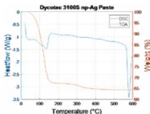
Figure 1: b) TGA and DSC of the printed Ag nanoparticle ink.
