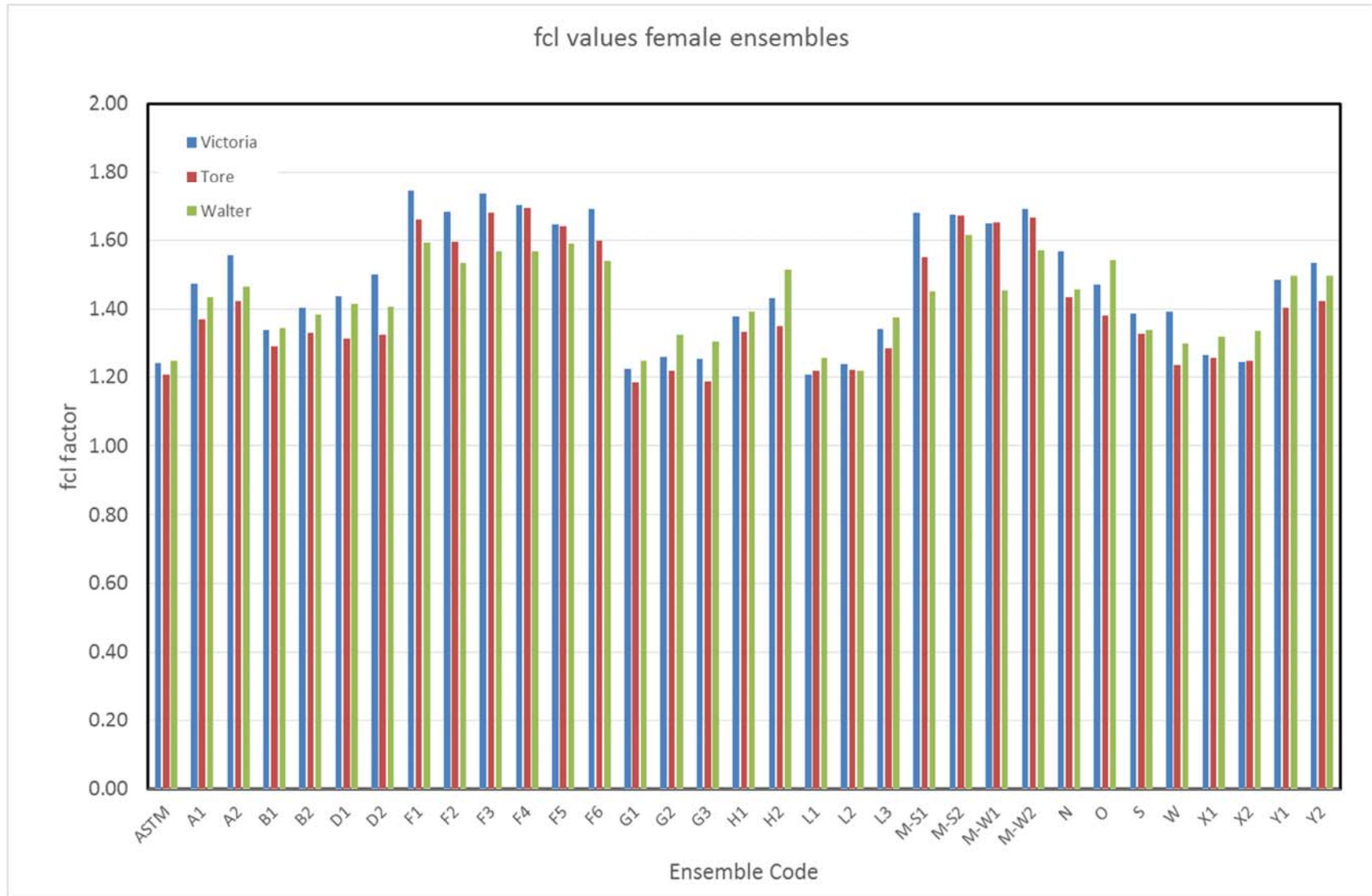
Figure 13, Comparison of measurements of f_{cl} for Female ensembles on Victoria, Tore and Walter
