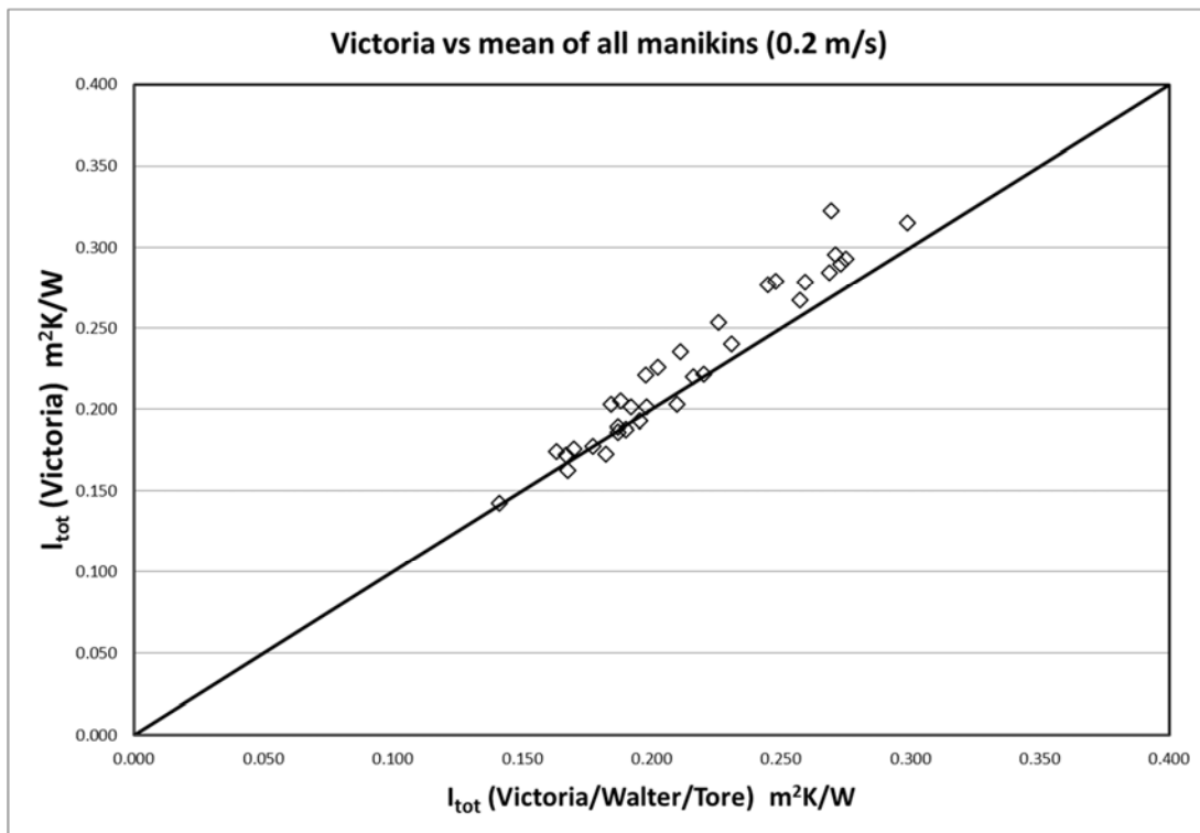
Figure 5; comparison of Female data measured on Victoria to the mean of three manikins: Victoria, Walter and Tore on which the same female ensemble was measured.
