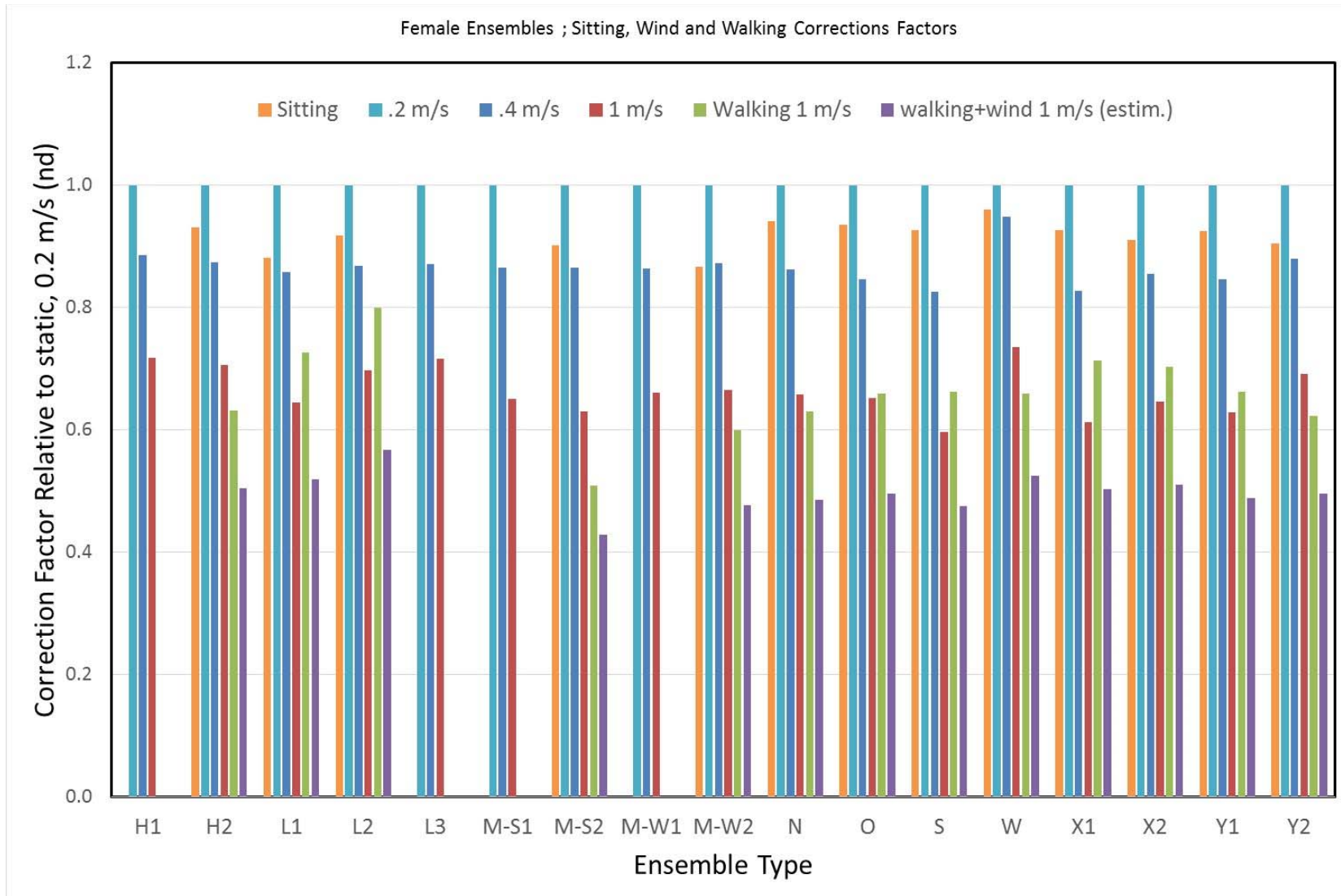
Figure 16; Correction Factors for the effects of air velocity (Victoria/Newton), and walking and sitting (Tore) on total clothing insulation i_{r} . To obtain the insulation value for sitting, walking or different air speeds, the static 0.2 \text{ m}\cdot\text{s}^{-1} value needs to be multiplied with the respective factor shown here. [NOTE: walking was measured in the same relative air speed as standing and sitting. Hence this only represents the effect of the pumping effect of the movement. It does NOT include the effect of the air speed generated by moving forward; an estimate of the combined effect is provided based on data by Havenith & Nilsson, 2004].
