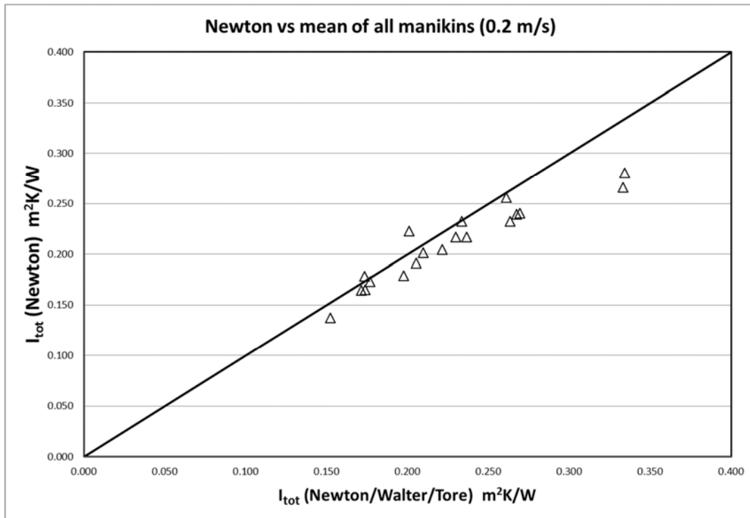
Figure 6; comparison of Male data measured on Newton to the mean of three manikins: Newton, Walter and Tore on which the same male ensemble was measured.
