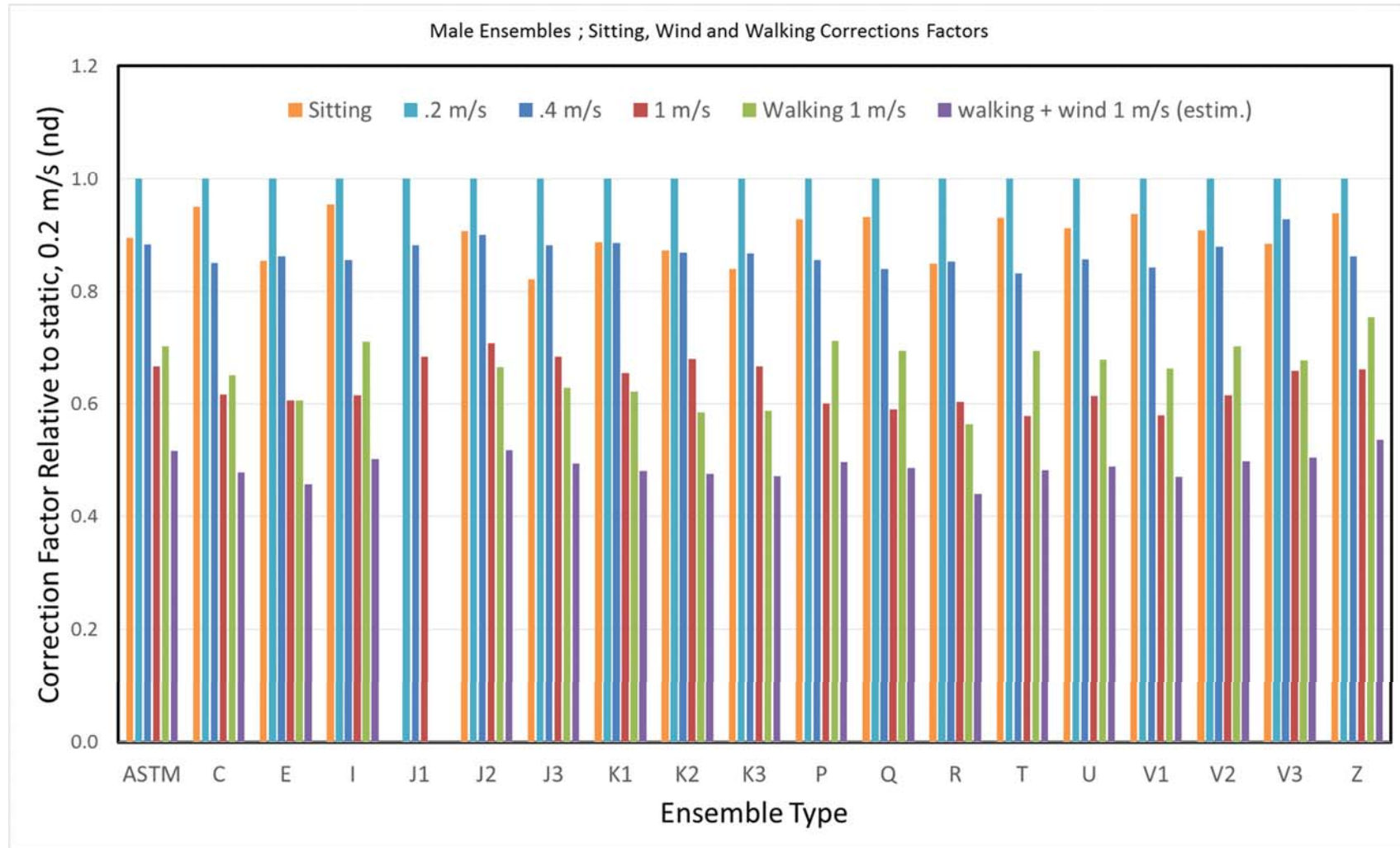
Figure 17; Correction Factors for the effects of air velocity (Victoria/Newton), and walking and sitting (Tore) on total clothing insulation i_r . To obtain the insulation value for sitting, walking or different air speeds, the static 0.2 \text{ m}\cdot\text{s}^{-1} value needs to be multiplied with the respective factor shown here. [NOTE: walking was measured in the same relative air speed as standing and sitting. Hence this only represents the effect of the pumping effect of the movement. It does NOT include the effect of the air speed generated by moving forward; an estimate of the combined effect is provided based on data by Havenith & Nilsson, 2004].
