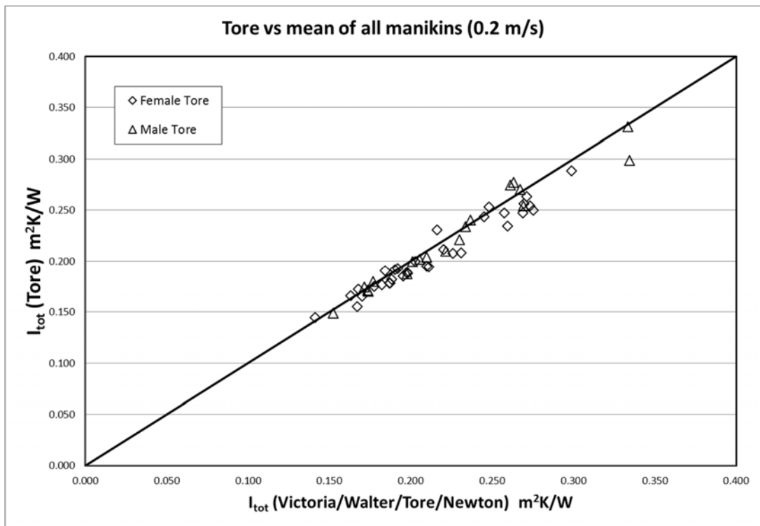
Figure 7; comparison of data measured on Tore to the mean of three manikins: Victoria/Newton, Walter and Tore on which the same ensemble was measured.
