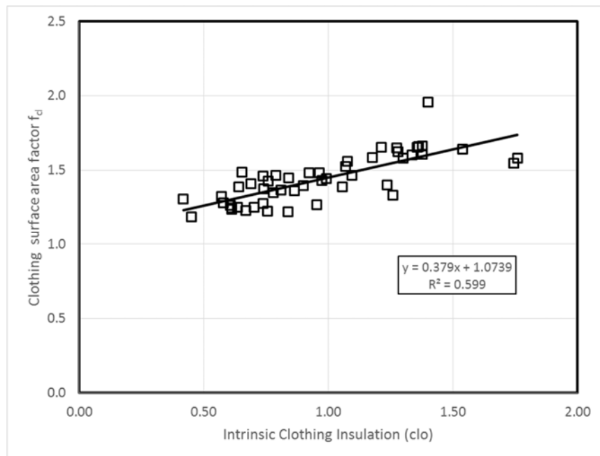
Figure 12, Relationship between clothing area factor f_{cl} as measured according to appendix D, and intrinsic clothing insulation I_{cl} calculated using this f_{cl} value (see equation (2)).
