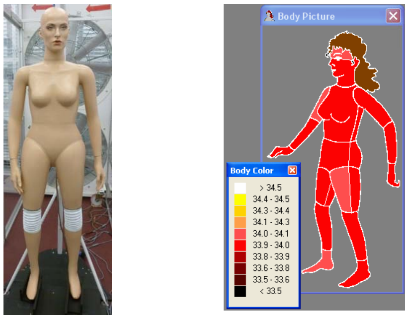
Figure 1; Female shaped Thermal Manikin used at Loughborough University ('Victoria') with zone distribution (right).
