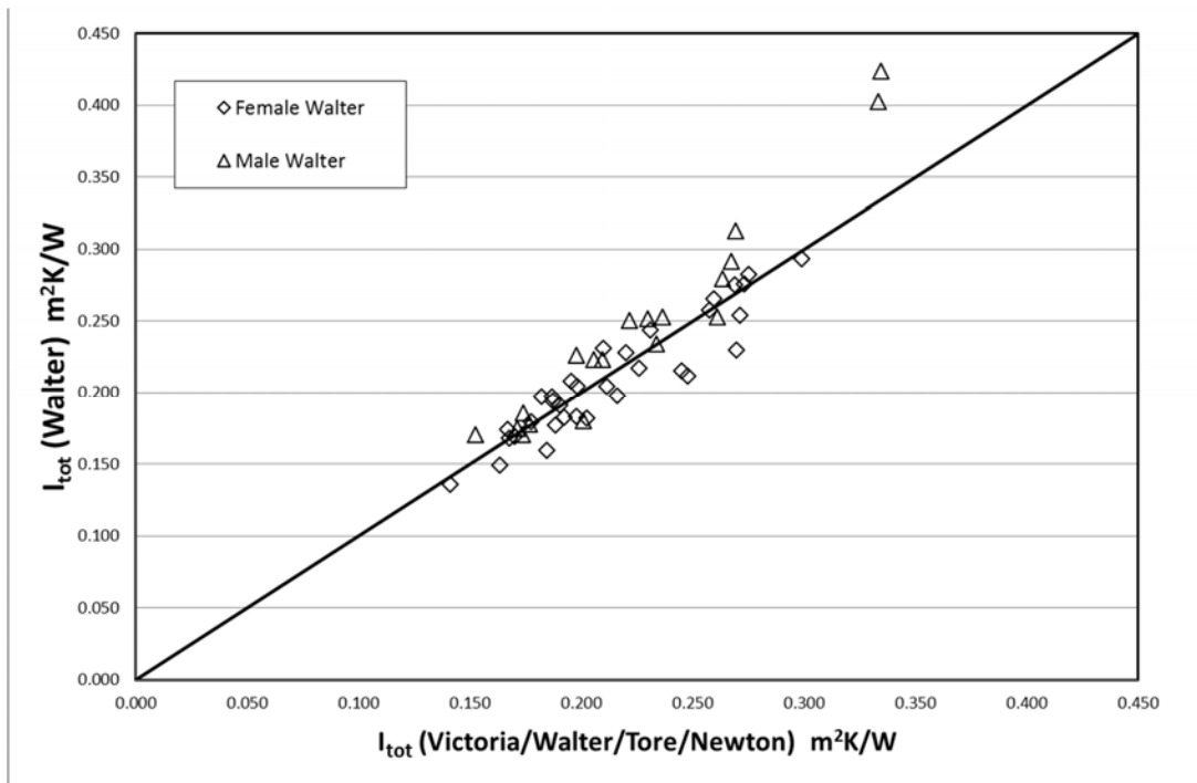
Figure 8; comparison of data for total clothing insulation I_{tot} measured on Walter (corrected to 0.2 m/s air speed) to the mean of three manikins: Victoria or Newton, and Walter and Tore on which the same ensemble was measured..
