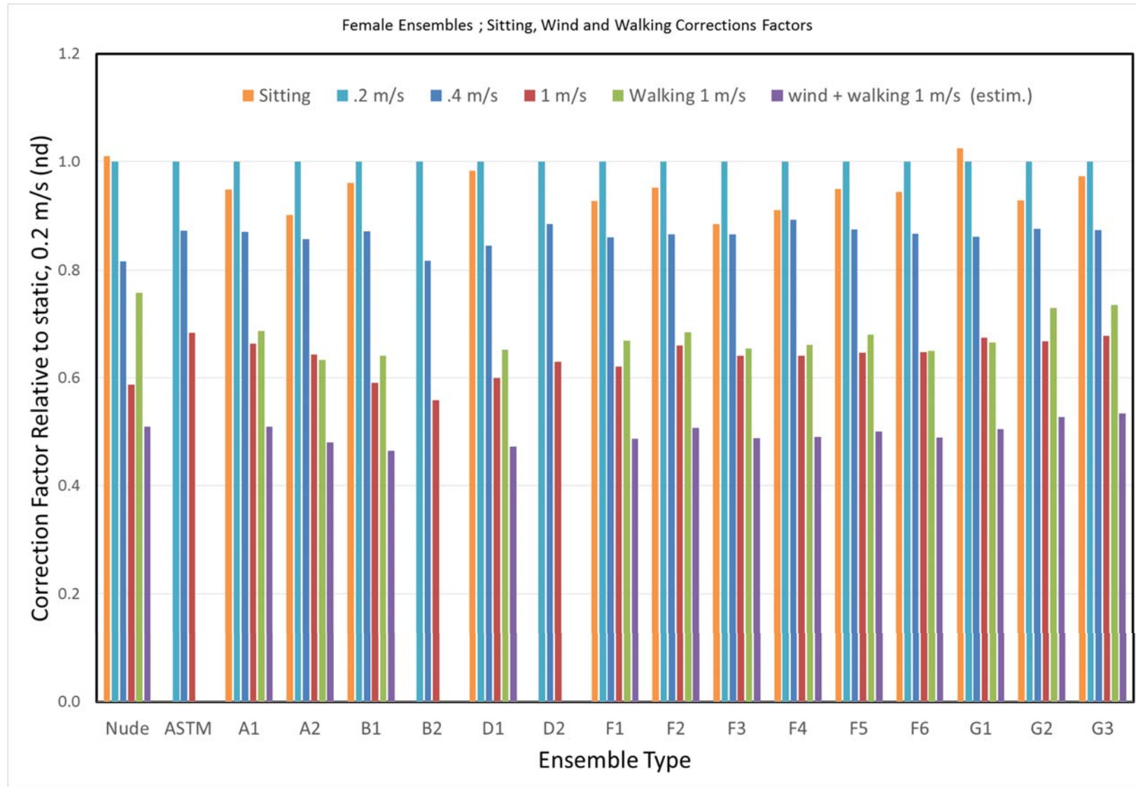
Figure 15; Correction Factors for the effects of air velocity (Victoria/Newton), and walking and sitting (Tore) on total clothing insulation i_T . To obtain the insulation value for sitting, walking or different air speeds, the static 0.2 \text{ m}\cdot\text{s}^{-1} value needs to be multiplied with the respective factor shown here. [NOTE: walking was measured in the same relative air speed as standing and sitting. Hence this only represents the effect of the pumping effect of the movement. It does NOT include the effect of the air speed generated by moving forward; an estimate of the combined effect is provided based on data by Havenith & Nilsson, 2004].
