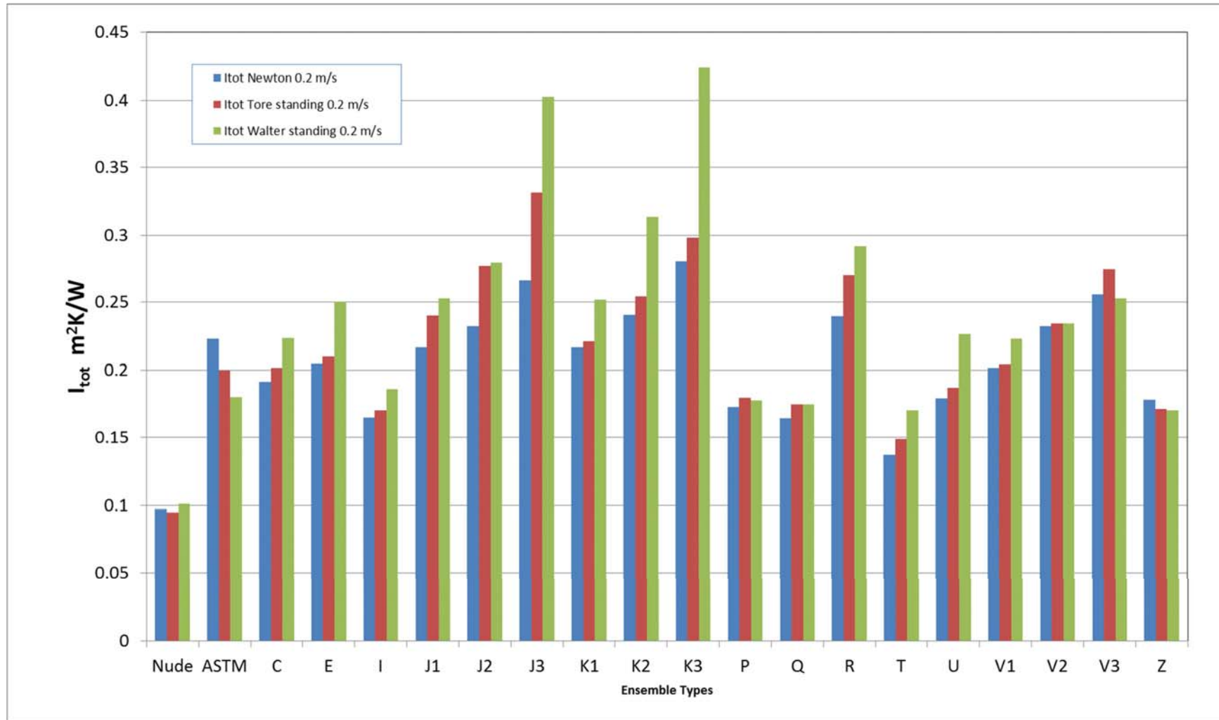
Figure 10; Comparison of measurements of Male ensembles on Newton, Tore and Walter.
