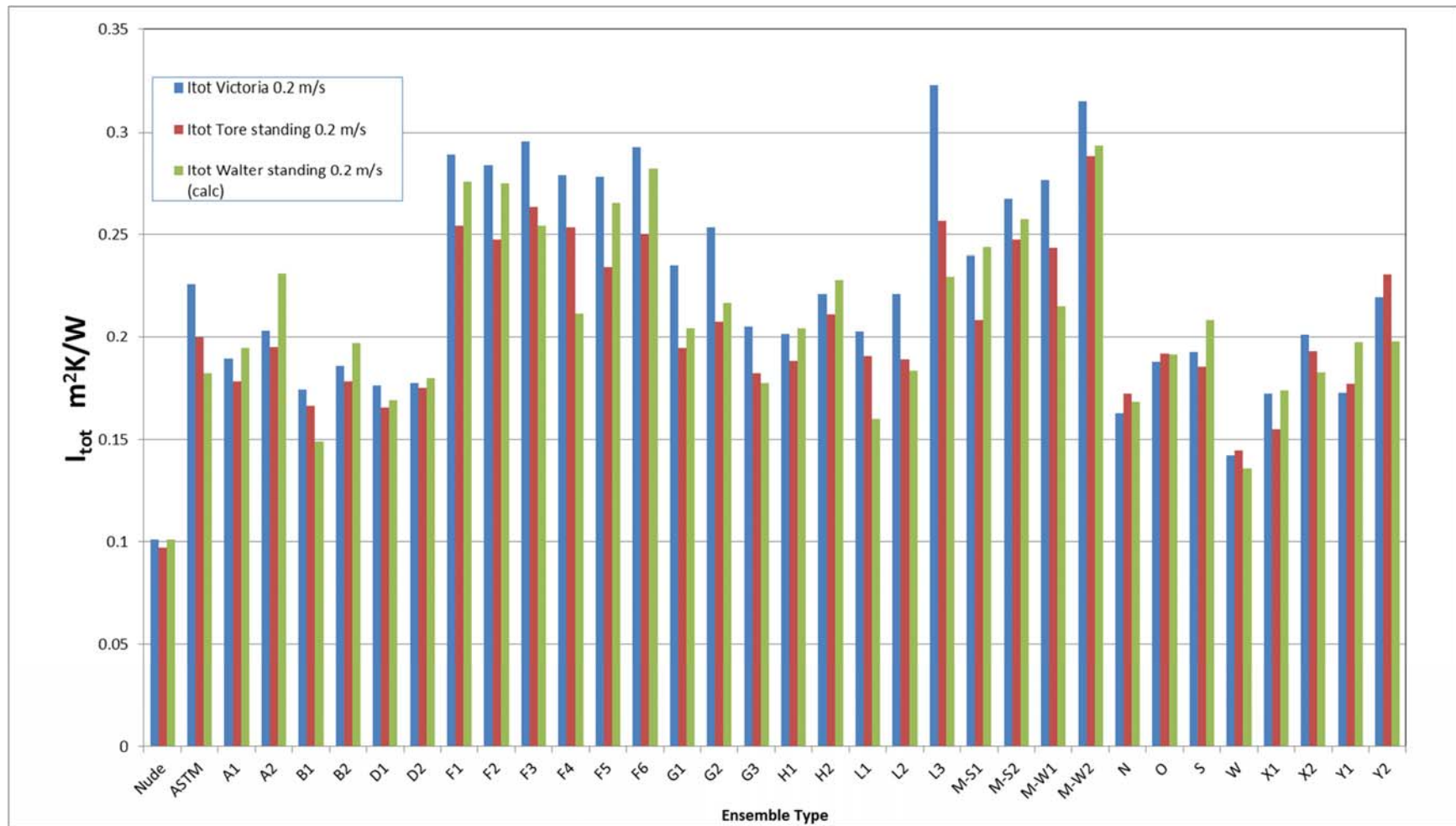
Figure 9; Comparison of measurements of Female ensembles on Victoria, Tore and Walter.
