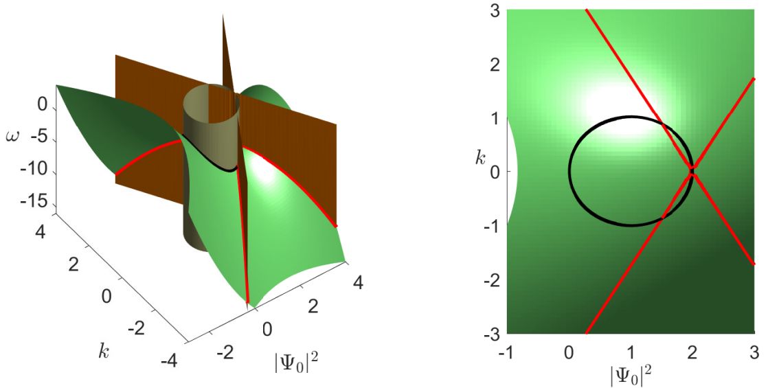
Figure 2: An example of the surfaces defined in (4.7) for \alpha = 4 . The surfaces corresponding to these conditions are coloured green, grey and orange respectively. The intersections between the second and third conditions with the first are highlighted by the black and red lines respectively. The second image shows the intersection between these lines from above and thus the points where the mKP-KD + equation emerges.
