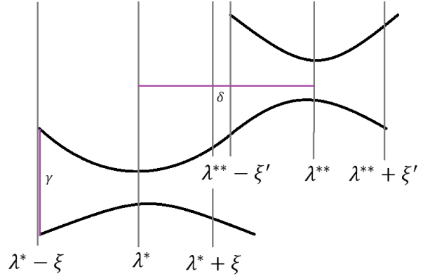
FIG. 1: 2 anticrossings in a close vicinity of each other.
