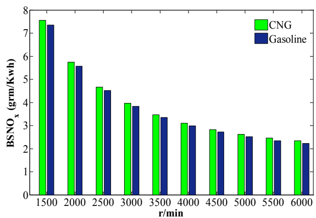
Figure 19. Comparison \text{BSNO}_x for gasoline and CNG fuels in various engine speeds
