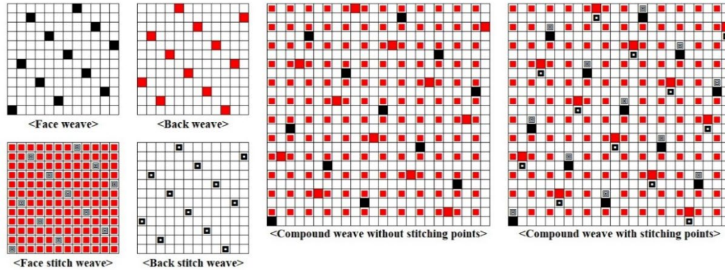
Figure 13: Double-cloth weave structure with or without stitching points
