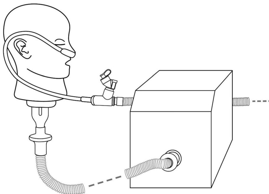
Fig. 2 Tracheal Dose test setup with high flow nasal cannula, showing the adult head model attached to the breathing simulator
