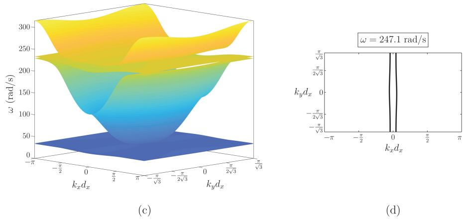
Figure 6: (a) Band diagram of the periodic system in Fig. 4 with \Omega = 0 , calculated along the path \Gamma XMY\Gamma illustrated in (b). (c) Dispersion surfaces of the system, computed numerically. (d) Slowness contours for \omega = 247.1 rad/s.
