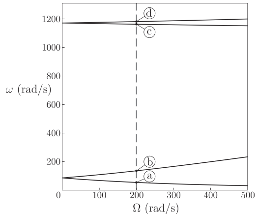
Figure 3: Eigenfrequencies corresponding to the flexural motion of the chiral multi-structure in Fig. 2 versus the gyricity \Omega . The frequencies \omega_a , \omega_b , \omega_c and \omega_d are computed for \Omega = 200 rad/s.
