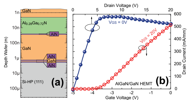
Fig. 1. (a) Schematic cross-section of the device epi-structure grown on a Si-HP (111) substrate. The source-to-drain distance and the gate width are 5 \mu\text{m} and 100 \mu\text{m} , respectively. (b) I_{DS} - V_{DS} and I_{DS} - V_{GS} characteristics at V_{GS} = 0 V and V_{DS} = 20 V obtained from the \text{Al}_{0.28}\text{Ga}_{0.72}\text{N}/\text{GaN} HEMT. The threshold voltage ( V_{th} ) is -3.5 V.
