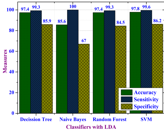
FIGURE 3: Performance Evaluation of Classifiers using LDA for Dimensionality Reduction
