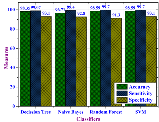
FIGURE 2: Performance Evaluation of Classifiers without Dimensionality Reduction
