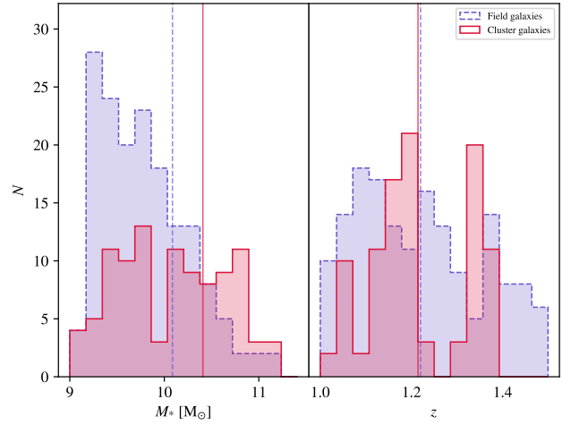
Figure 4. The stellar mass ( left ) and redshift ( right ) distributions for the field (dashed purple) and cluster (solid crimson) samples. The vertical lines represent the mean stellar mass and mean redshift of the cluster and field galaxy populations.
