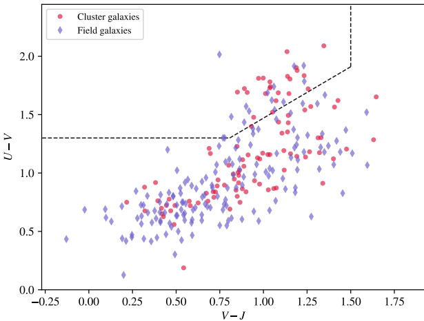
Figure 3. UVJ -diagram of [\text{O II}] emitters with classifications from Muzzin et al. (2013) for 1 < z < 4 (adapted from Williams et al. 2009) where quiescent galaxies are above the dashed line in the upper left region, and star-forming galaxies are below the dashed line.
