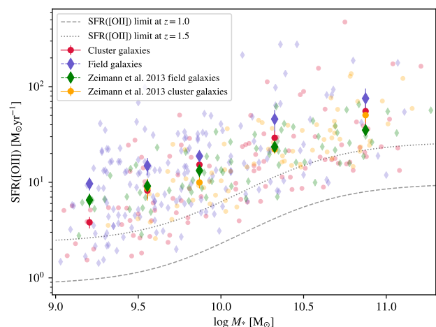
Figure B2. [\text{O II}] -derived main sequence of star formation of cluster galaxies versus field galaxies in the GOGREEN fields, along with the \text{H}\alpha -derived main sequence from Zeimann et al. (2013). The solid purple and crimson markers signify the mean GOGREEN field SFRs and the GOGREEN cluster galaxy SFRs in each stellar mass bin respectively. The solid orange and green markers signify the mean Zeimann et al. (2013) field SFRs and the Zeimann et al. (2013) cluster galaxy SFRs in each stellar mass bin respectively. The GOGREEN field SFRs have been corrected using the cosmic SFR vs. z relation of Equation 7 in order to match the mean redshift of GOGREEN cluster galaxies within each stellar mass bin. The error bars represent the bootstrap standard error from bootstrap resampling the data within each bin. The dashed and dotted grey lines represent the SFRs that correspond to the 80% flux completeness limit at z = 1.0 and z = 1.5 respectively.
