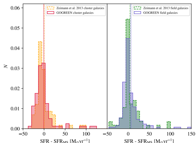
Figure B1. [\text{O II}] -derived GOGREEN cluster (solid) \Delta\text{SFR}_{\text{MS}} distribution and \text{H}\alpha -derived Zeimann et al. (2013) cluster (dashed) \Delta\text{SFR}_{\text{MS}} distribution (left). GOGREEN field (solid) and Zeimann et al. (2013) field (dashed) \Delta\text{SFR}_{\text{MS}} distributions are shown on the right.
