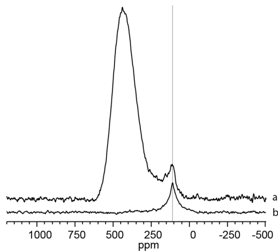
Figure 1. (a) ^{13}\text{C} NMR spectrum of \text{ZrC}_{1-x} , nominal \text{C}/\text{Zr} = 0.60 , sintered at 2000^\circ\text{C} (b) spectrum of precursor graphite located at \sim 113 ppm.
