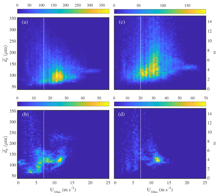
Figure 15. Properties of blowing-snow particle size distributions above sea ice as a function of the 10 m wind speed U_{10m} retrieved from fitting a two-parameter gamma probability density function (Eq. 5) to observations. Mean snow particle diameters \bar{d}_p ( = \alpha \beta ) (a) at 29 m during ANT-XXIX/6 and 7 and (b) at < 0.2 m during ANT-XXIX/6. The shape parameter \alpha (c) at 29 m and (d) at < 0.2 m. The vertical line represents the observed mean snowdrift threshold wind speed U_t of 7.1 \text{ m s}^{-1} corresponding to u_{*t} of 0.37 \text{ m s}^{-1} . Data were binned into 50 bins in the x and y direction, with the colour indicating the sample density in each bin.
