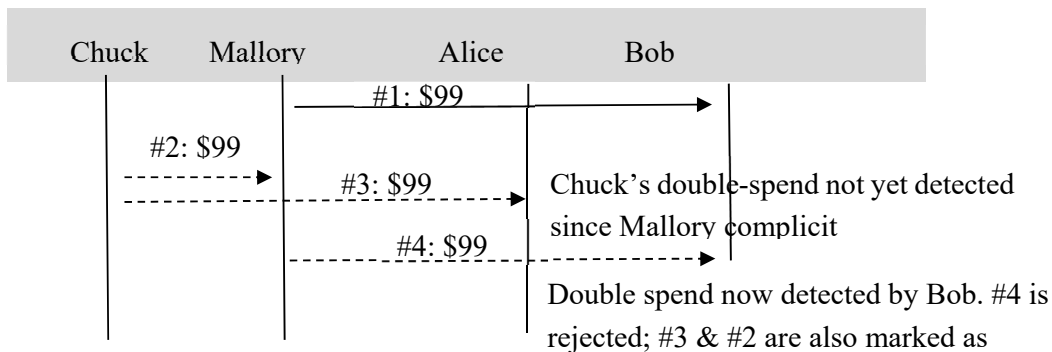
Figure 3. An example of transactions between two dishonest and two honest nodes, including attempted double-spending.
