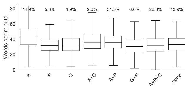
Figure 5: ITE method versus typing speed with 95% confidence intervals and percentage of participants in each group. P = Prediction; A = Autocorrection; G = Gesture.
