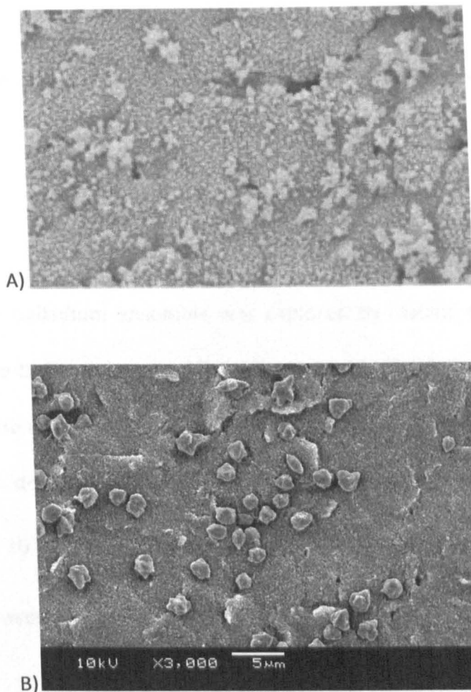
Figure 9.3. SEM images of the copper plated standard (A) and bespoke (B) screen-printed electrochemical platforms.
