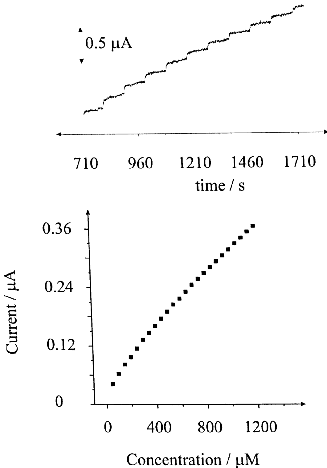
Figure 7.3: A typical amperometric response obtained at a 5% copper (II) oxide screen-printed electrochemical sensing platform resulting from 50 \mu\text{M} additions of glucose into a 0.1 M NaOH solution. The potential was held at + 0.6 V (vs. SCE). Also shown is the analysis of the current from the glucose additions.
