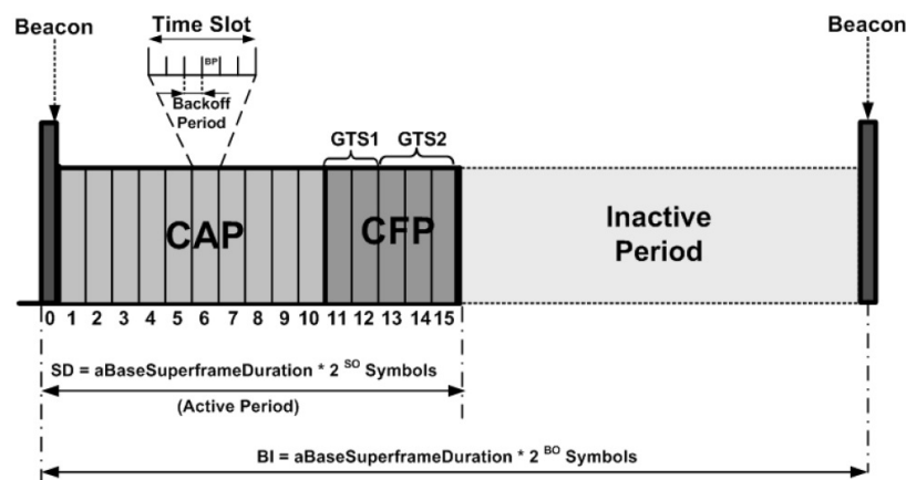
Figure 5. IEEE 802.15.4 superframe structure. CAP = Contention Access Period; CFP = Contention Free Period; GTS = Guaranteed Time Slot.
