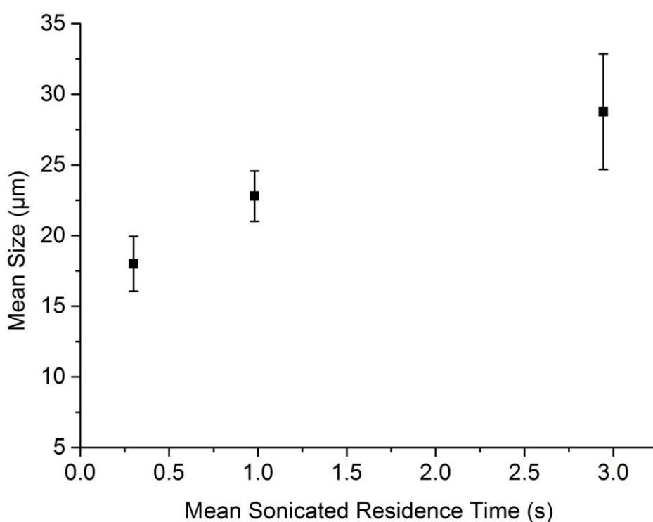
8 Figure 10: Effect of mean sonication residence time on mean crystal size in the 1.55 mm I.D. capillary. 9 The error bars represent one standard deviation in mean crystal size across different experimental 10 repeats (not the standard deviation of CSD which is given in supplementary information)
