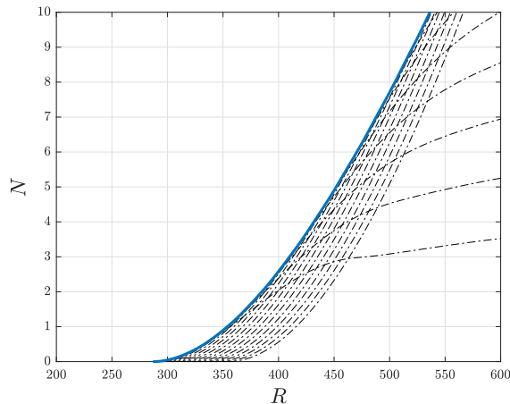
Figure 8: Amplitude ratio curve for \varepsilon = T_s = 0 . The dashed curves (--) represent amplitude ratio curves at fixed n ; the solid curve is the enveloping N -factor curve used to determine a transitional Reynolds number.
