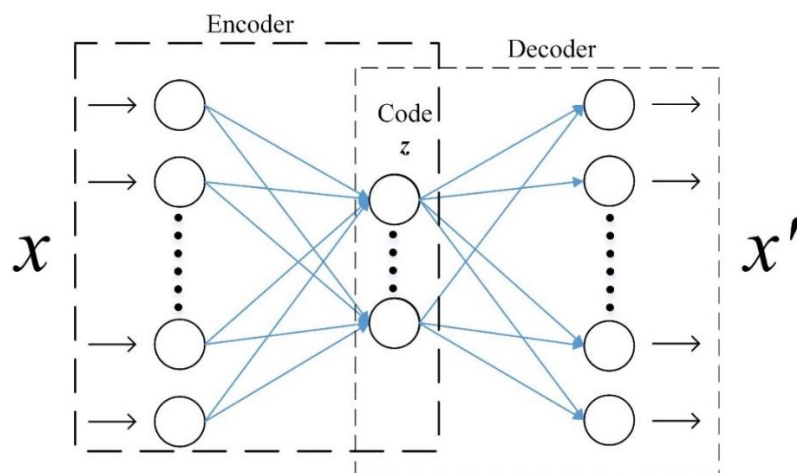
Figure 2. The structure of autoencoder
