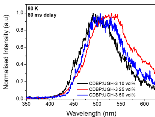
Figure 5.13 Phosphorescence spectra of vacuum deposited films of CDBP:UGH-3 at different CDBP vol%.
