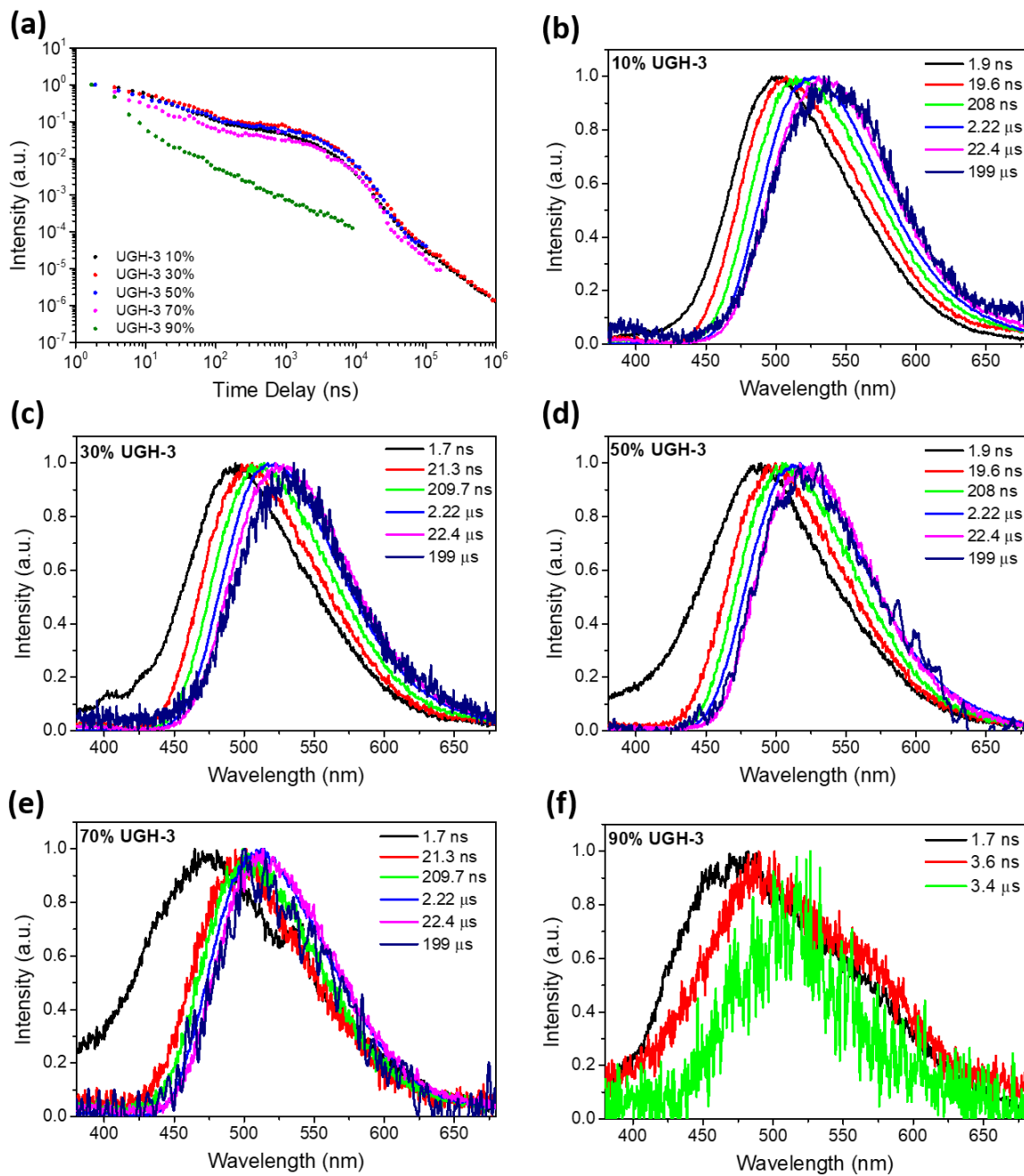
Figure 4.6 (a) Room temperature photoluminescence decays of evaporated TSBPA:PO-T2T exciplex films with increasing vol% of UGH-3. (b-f) Photoluminescence spectra of TSBPA:PO-T2T 1:1 ratio diluted in 10-90 vol% UGH-3 evaporated film at different delay times.
