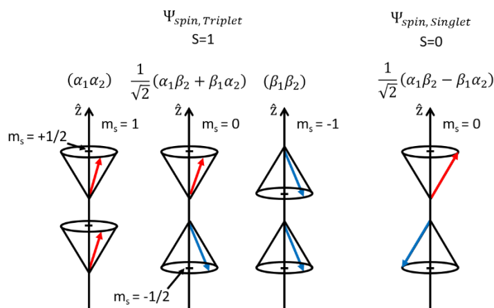
Figure 2.1 Spin Wavefunctions and cones of orientation of a two electron system, the index 1 and 2 refer respectively to electron 1 and 2. The red arrow indicates a spin-up electron with m_s = +1/2 while the blue arrow represents a spin down electron with m_s = -1/2 . At the top of the figure is reported the total spin of a triplet ( S = 1 and a singlet ( S = 0 ). Below (left) are reported the three symmetric spin wavefunctions of the triplet and (right) the anti-symmetric singlet wave function. The two cases where m_s = 0 are distinguished by the phase of the precession of the two electrons forming the triplet where are in-phase and forming the singlet where are out of phase thus describing a symmetric spin state (triplet) and an anti-symmetric spin state (singlet).
