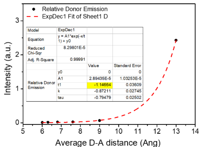
Figure 4.12 Distance dependence of residual donor emission (from Figure 4.4, UGH-3 series) corrected for differing exciplex PLQYs.
