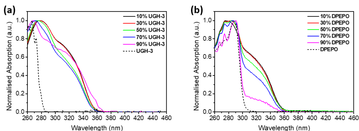
Figure 4.3 Absorption spectra of evaporated TSBPA:PO-T2T exciplex films with increasing vol% of (a) UGH-3 and (b) DPEPO.
