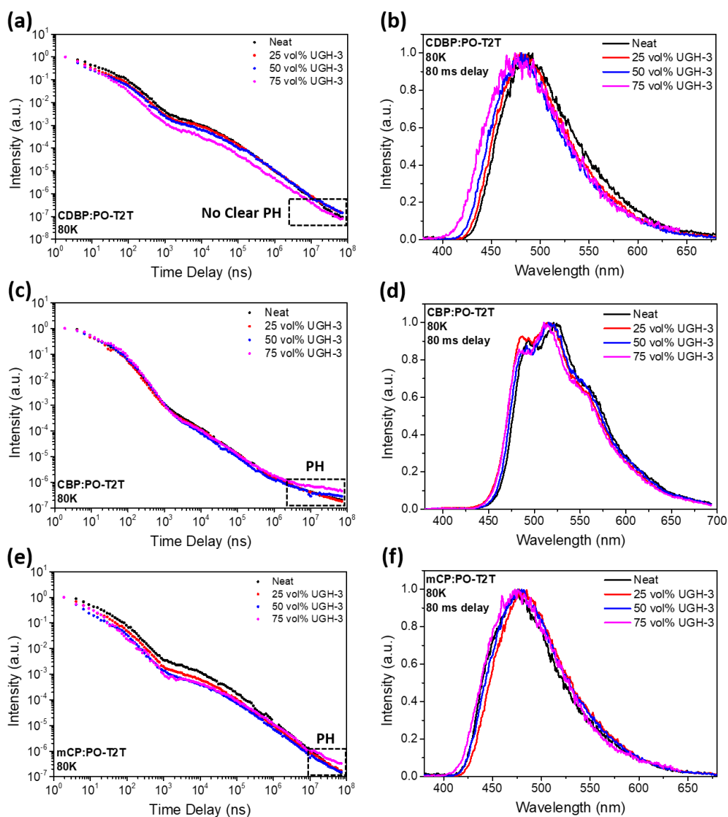
Figure 5.12 Left: Time resolved photoluminescence decays collected at 80K of (a) CDBP:PO-T2T (c) CBP:PO-T2T and (e) mCP:PO-T2T 1:1 vol% ratio and in different vol% of UGH-3. Right: PL spectra measured at 80K and 80 ms delay time and 10 ms integration time of (b) CDBP:PO-T2T (d) CBP:PO-T2T and (f) mCP:PO-T2T 1:1 vol% ratio and in different vol% of UGH-3
