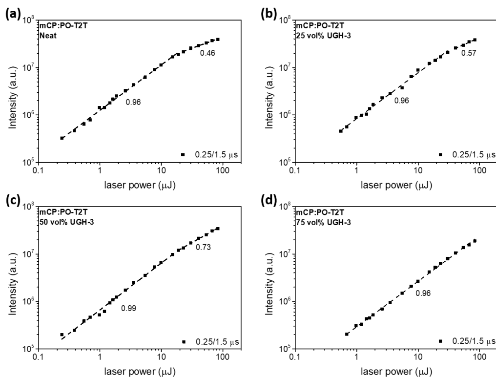
Figure 5.11 Linear fit of the of the integrated photoluminescence intensity vs the laser power measured at 0.25 \mu\text{s} delay and 1.5 \mu\text{s} integration time of mCP:PO-T2T 1:1 ratio evaporated films, (a) neat exciplex, (b) diluted in 25vol% UGH-3, (c) diluted in 50vol% UGH-3, (d) diluted in 75vol% UGH-3.
