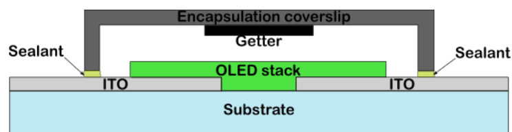
Figure 3.6 Scheme of an encapsulated OLED device for lifetime testing.
