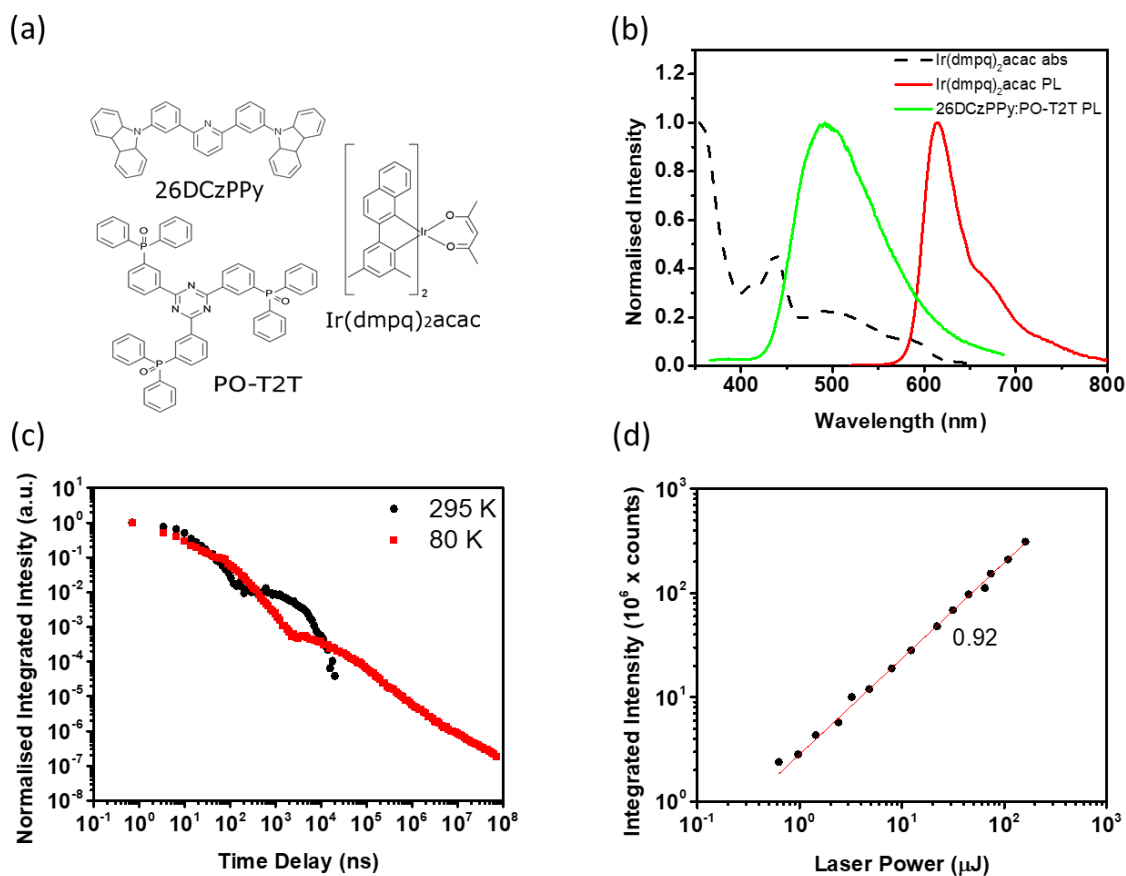
Figure 7.1 (a) Molecular structure of the exciplex forming donor (26DCzPPy), acceptor (PO-T2T) and phosphorescent emitter (Ir(dmpq) 2 acac) used in this study. (b) The normalised absorption and PL spectra of Ir(dmpq) 2 acac and 26DCzPPy:PO-T2T exciplex. (c) Time resolved fluorescence decay curves of the exciplex blend at 80 K and 295 K. (d) Integrated area as a function of the laser excitation (355 nm) of 26DCzPPy:PO-T2T exciplex blend.
