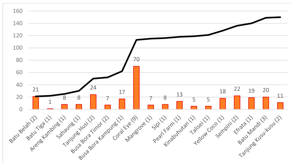
Figure 25. Species accumulation curve (black line) and number of species per locality (red bars). Numbers in brackets after the locality name indicate the number of sampling events at that particular site. Note the high number of sampling events at the locality Coral Eye.
