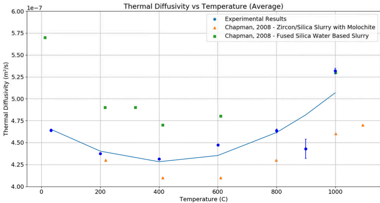
Figure 1. Comparative plot between the experimental thermal diffusivity profile and results published in literature as a function of temperature
