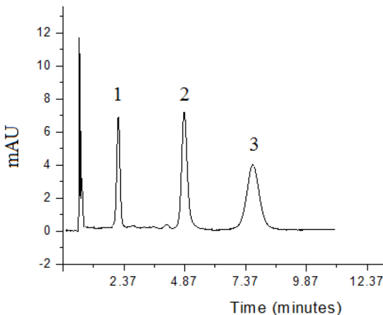
Figure 2: Chromatogram of the three pesticides analyzed in this study. (1) imidacloprid, (2) \beta -cyfluthrin, (3) abamectin.
