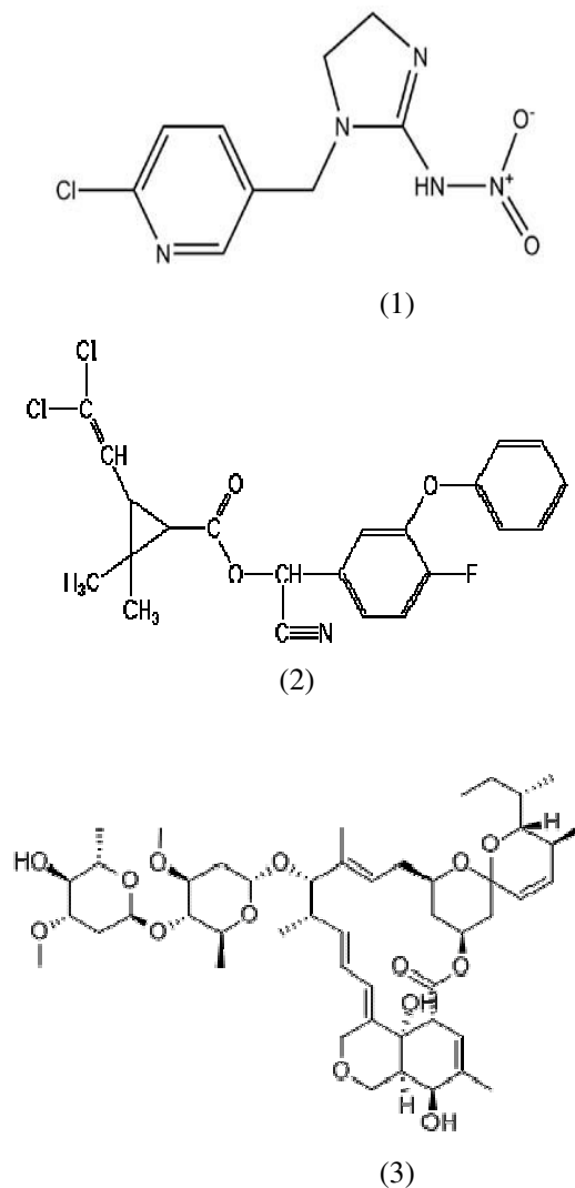
Figure 1: Structures of the three pesticides analyzed in this study: (1) imidacloprid (2) \beta -cyfluthrin (3) abamectin.
