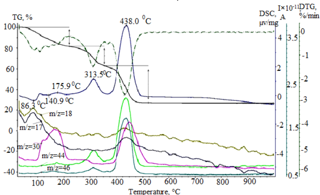
Figure 3. The thermal analysis data of the FFS dried at 60 \text{ }^\circ\text{C} with mass spectrometry data of the products of its decomposition.
